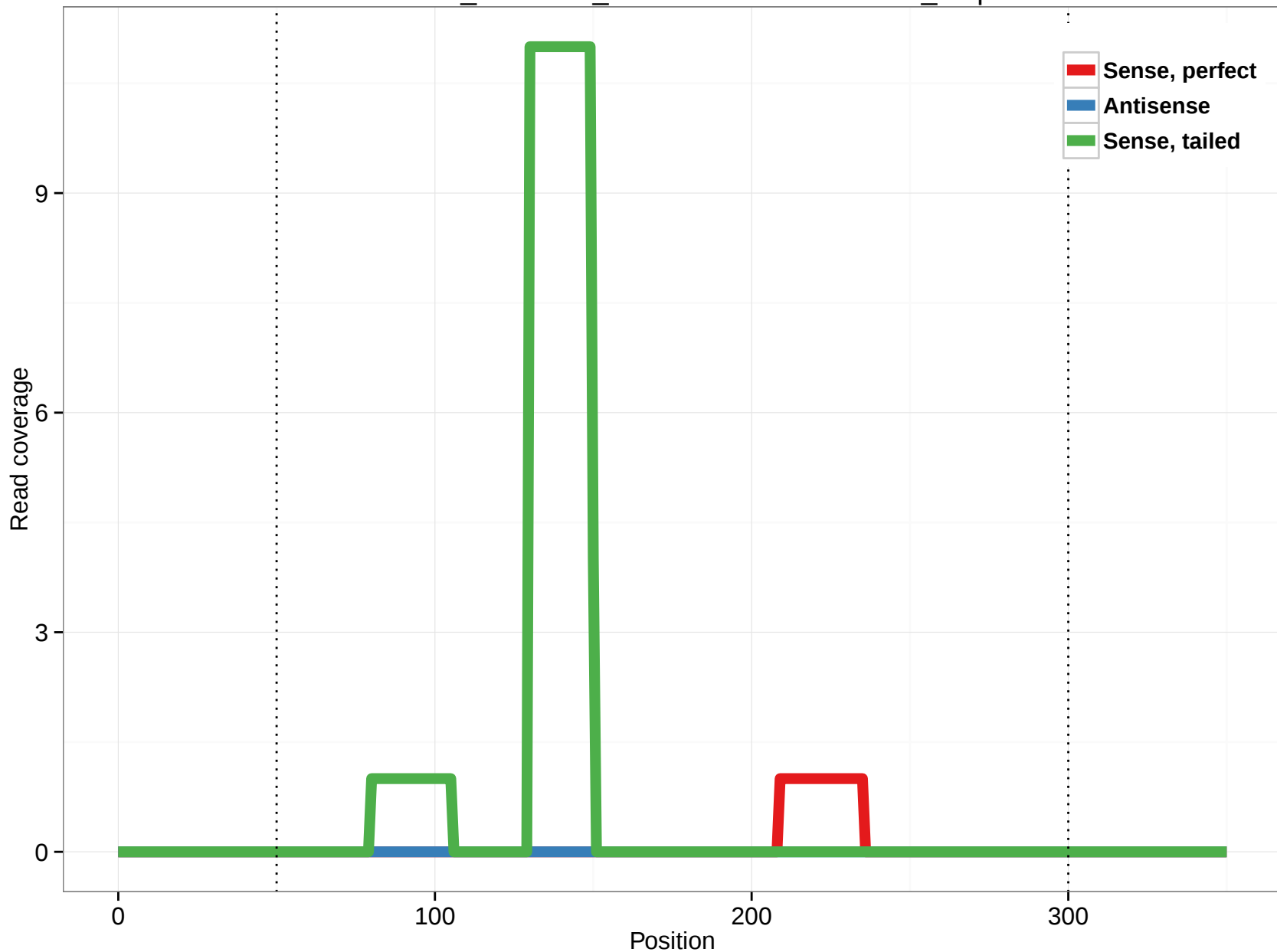
ornAna1_ensGene_ENSOANT00000009650_7.3p
