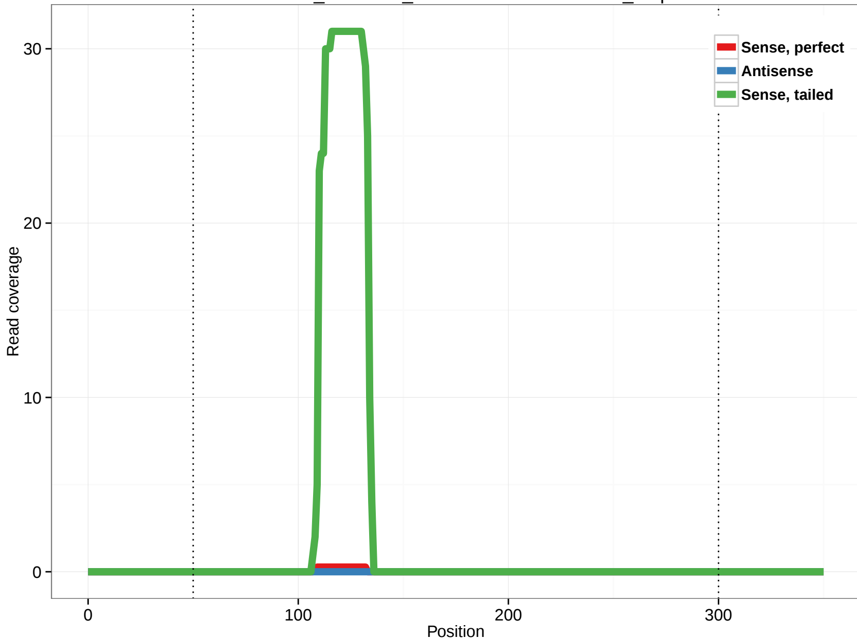
ornAna1_ensGene_ENSOANT00000009489_6.3p
