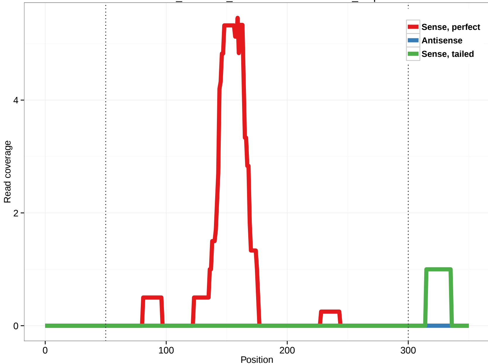
ornAna1_ensGene_ENSOANT00000009426_8.5p
