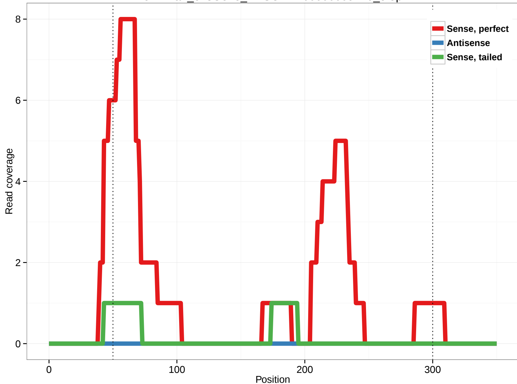
ornAna1_ensGene_ENSOANT00000009410_5.5p
