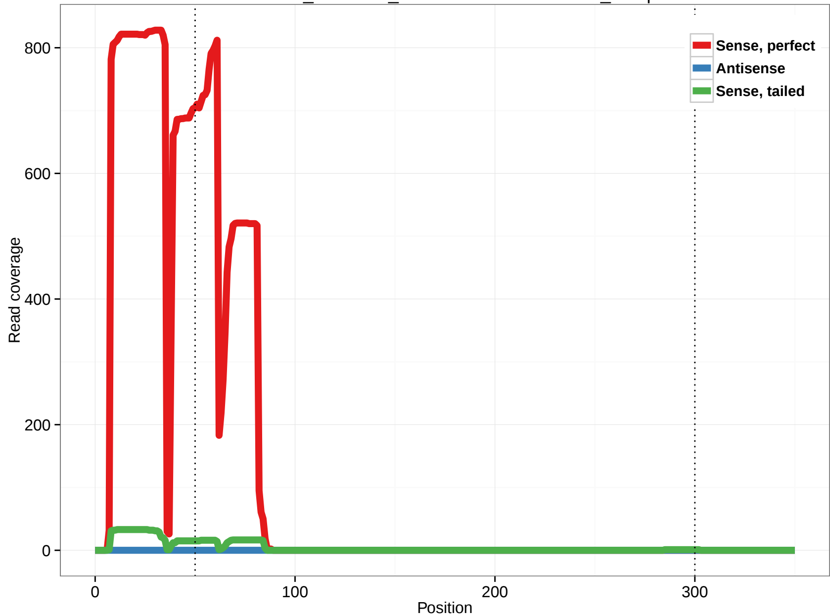
ornAna1_ensGene_ENSOANT00000009397_19.5p
