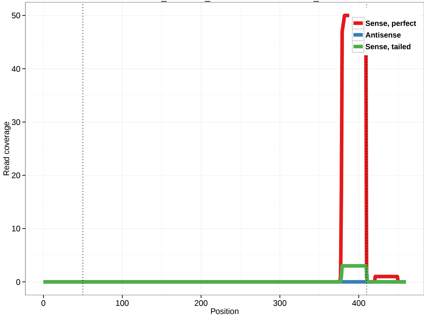
ornAna1_ensGene_ENSOANT00000009320_3
