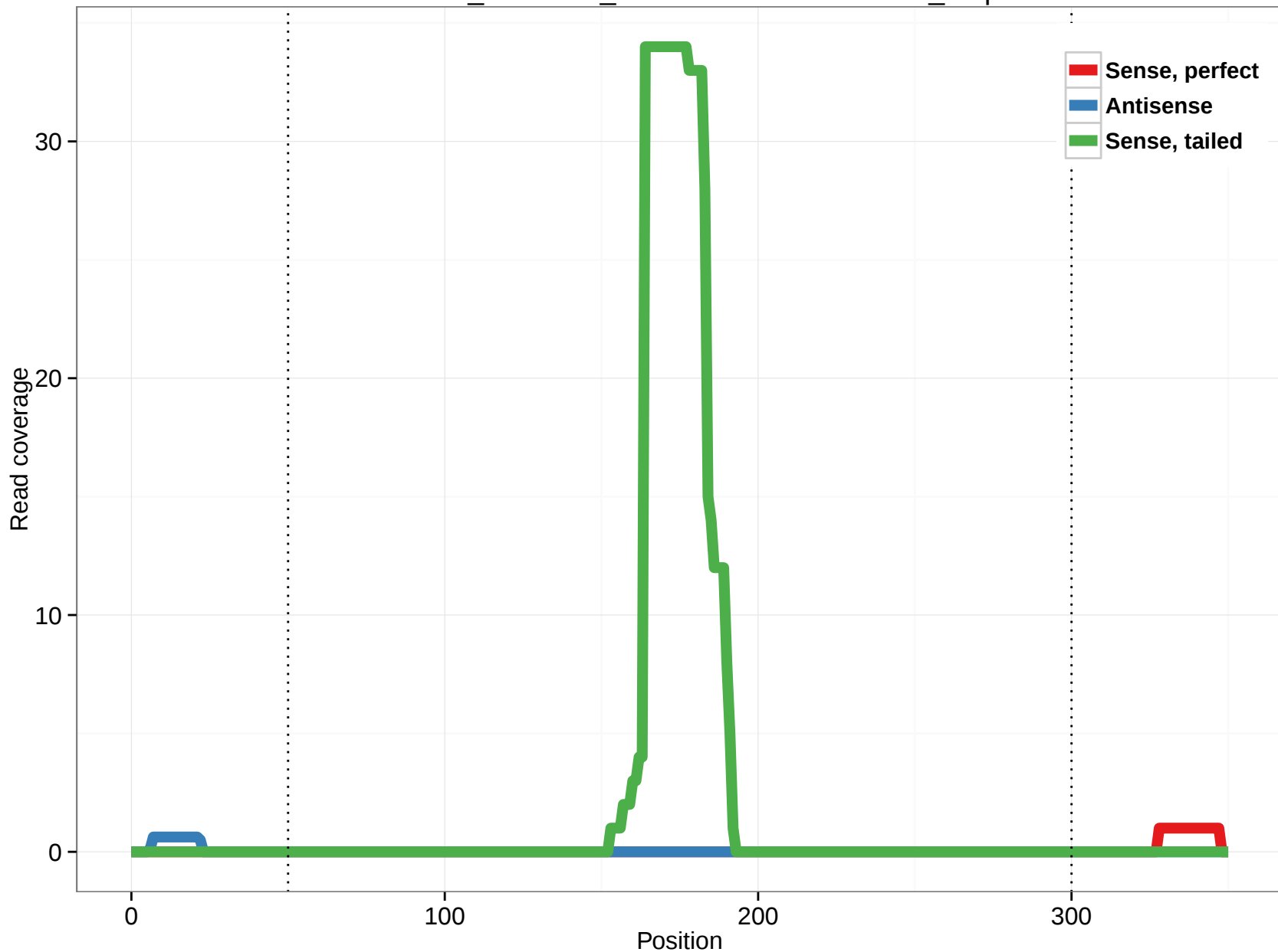
ornAna1_ensGene_ENSOANT00000009264_6.3p
