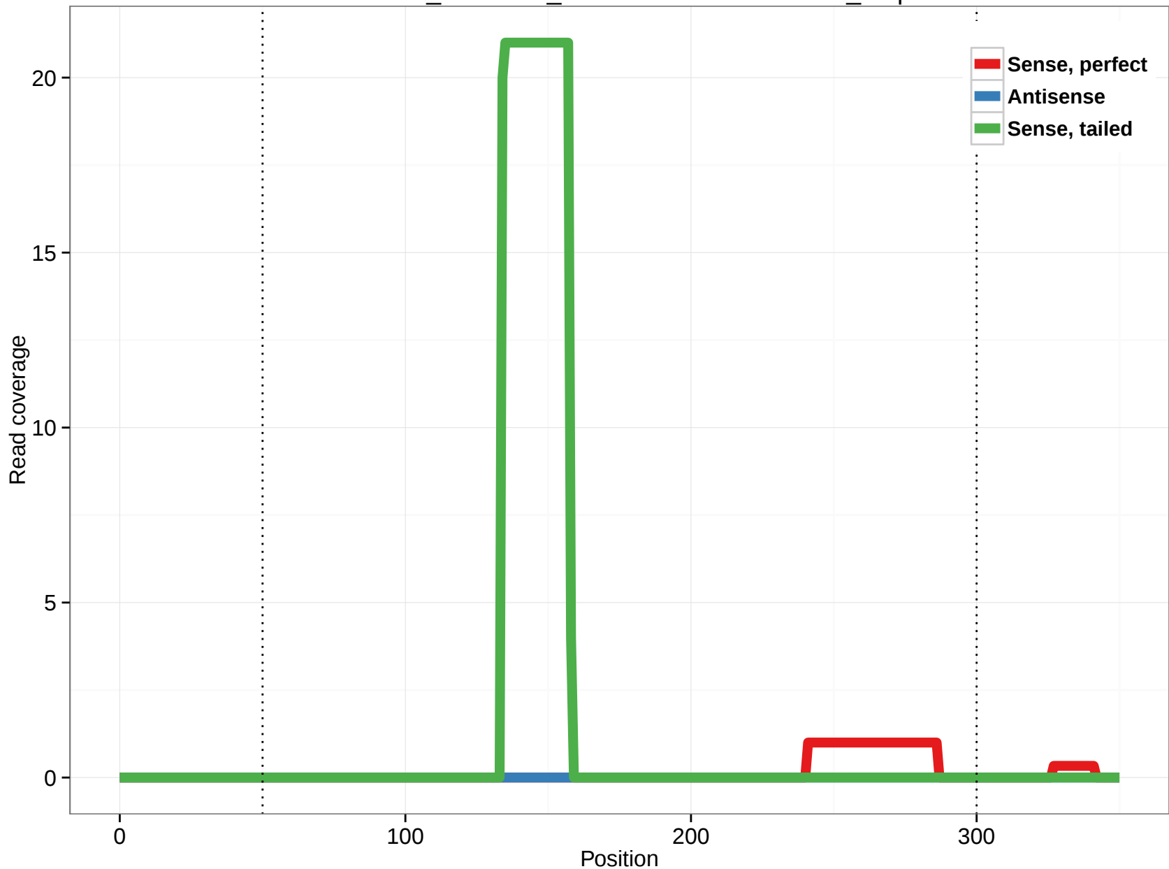
ornAna1_ensGene_ENSOANT00000009232_2.3p
