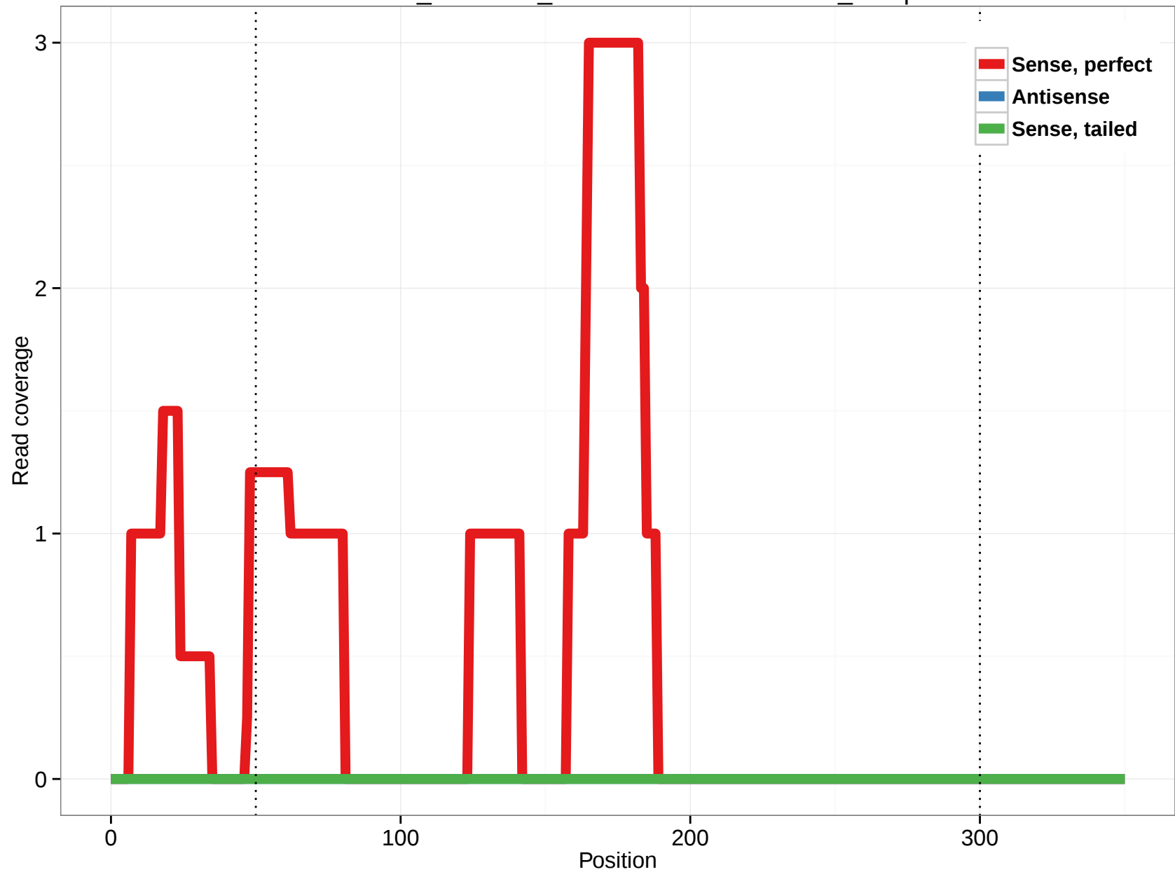
ornAna1_ensGene_ENSOANT00000009128_11.5p
