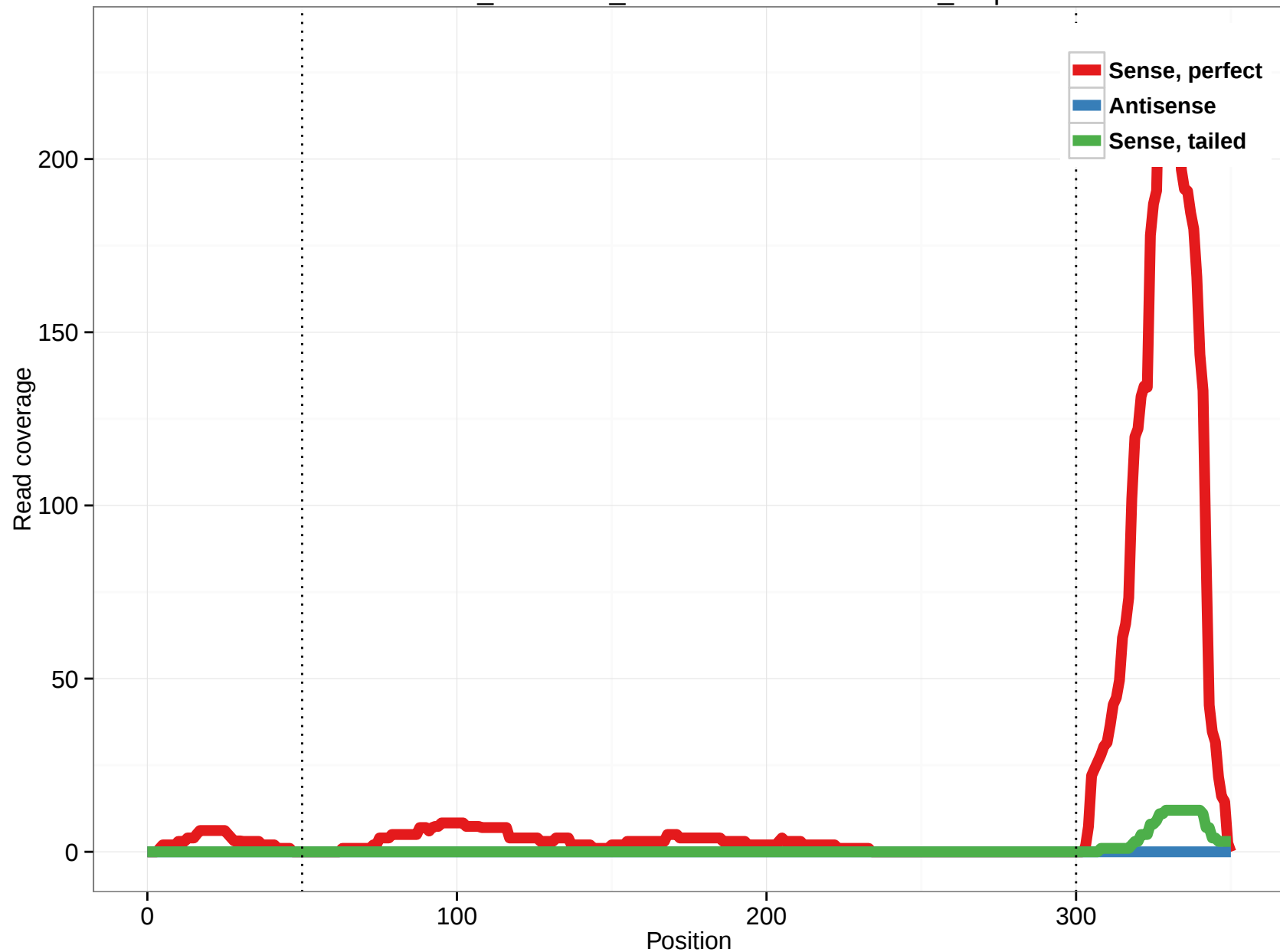
ornAna1_ensGene_ENSOANT00000009121_9.3p
