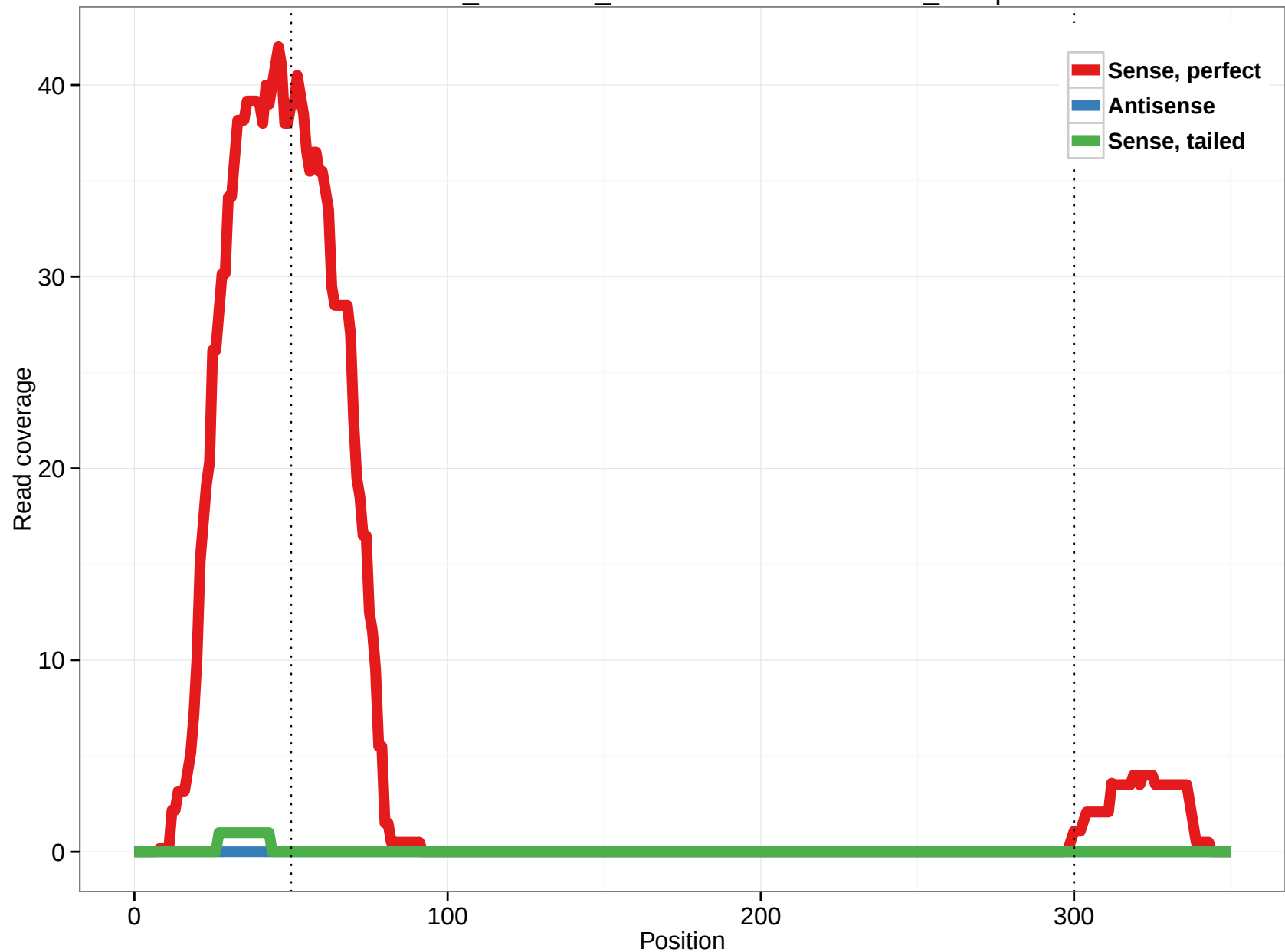
ornAna1_ensGene_ENSOANT00000009075_13.3p
