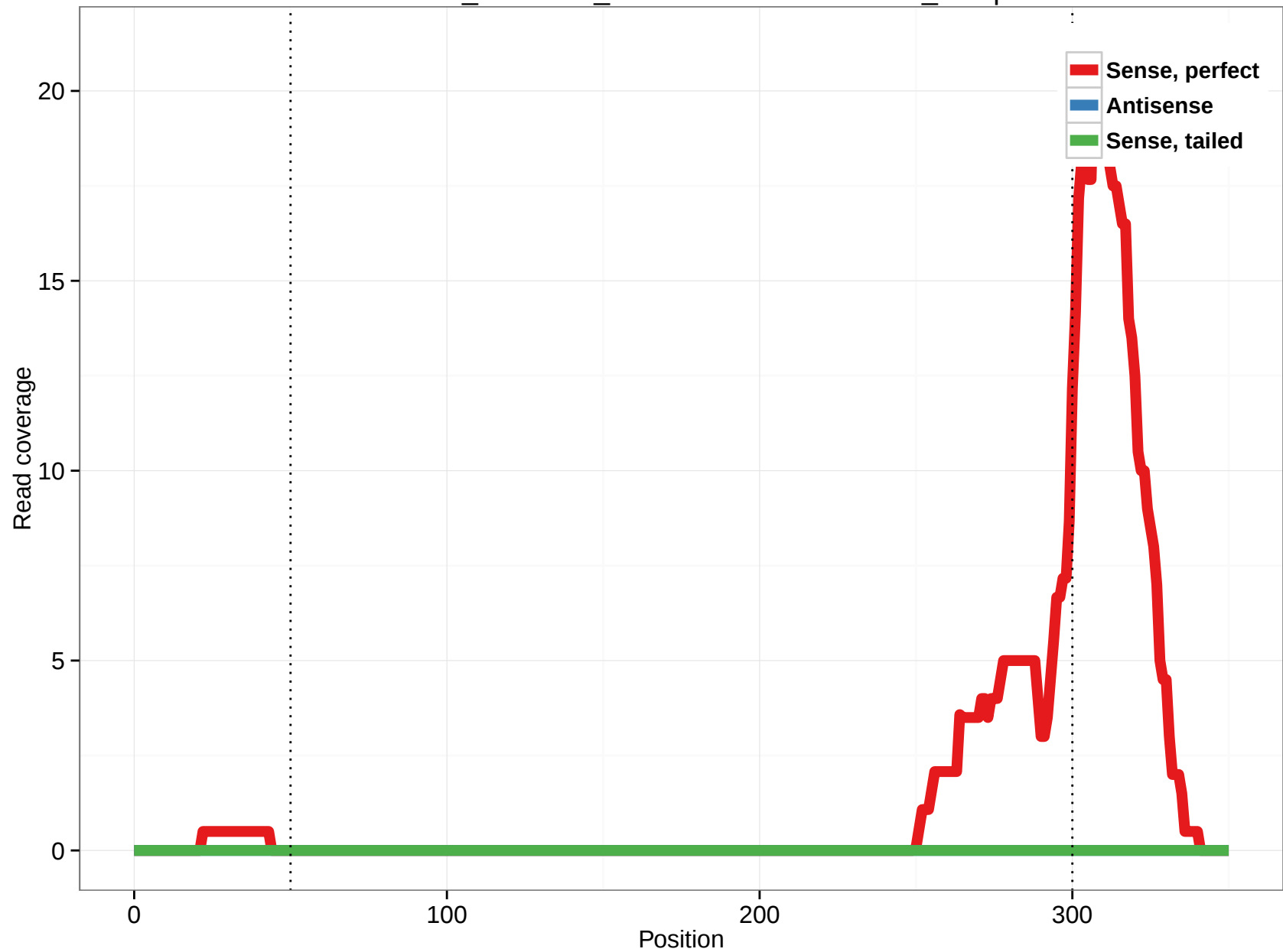
ornAna1_ensGene_ENSOANT00000009075_12.5p
