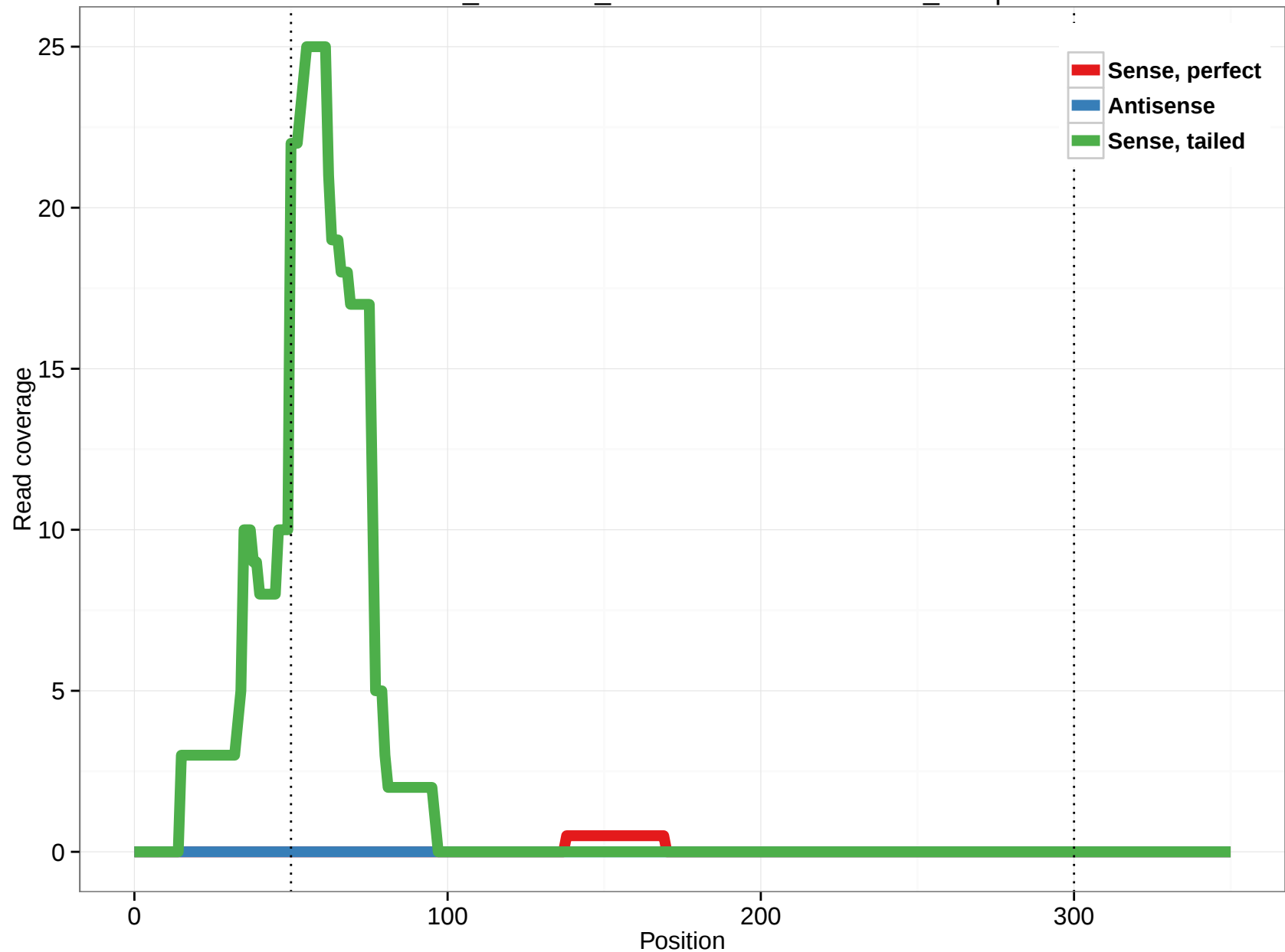
ornAna1_ensGene_ENSOANT00000009036_13.3p
