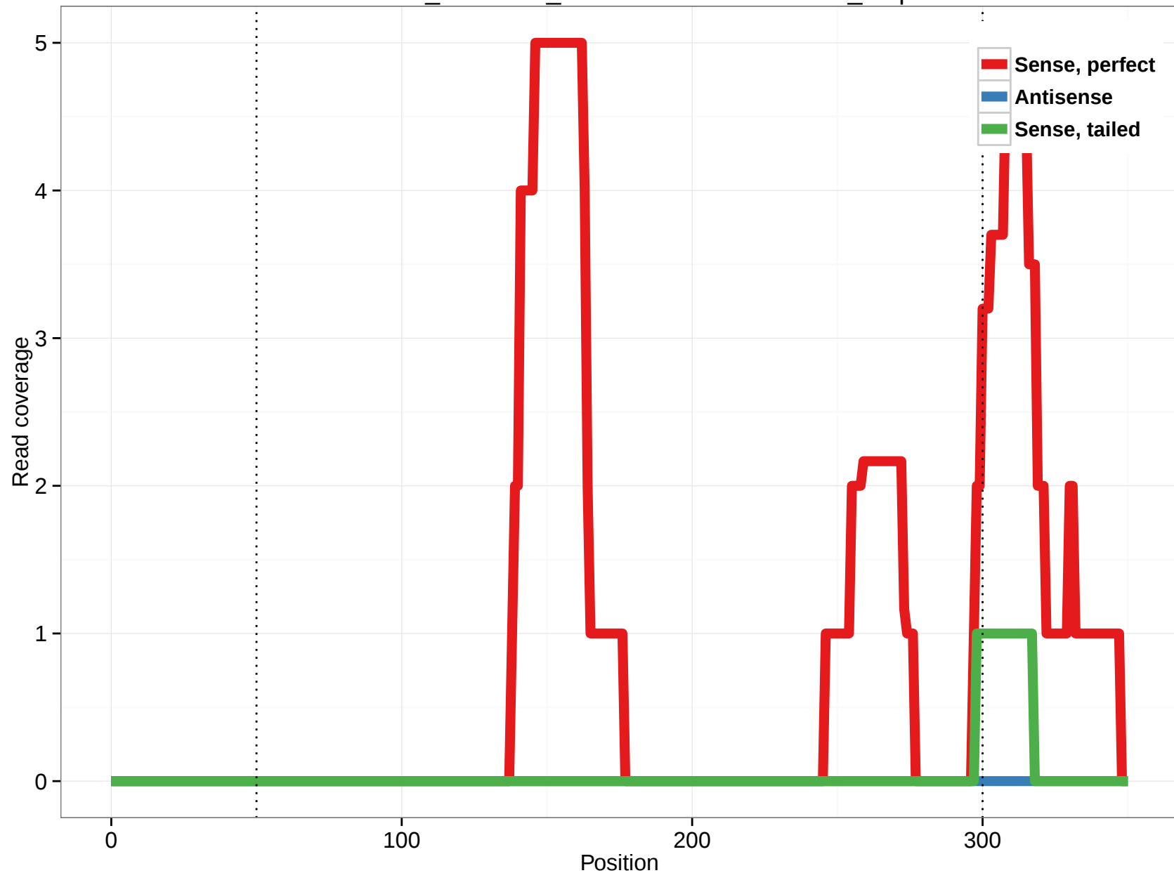
ornAna1_ensGene_ENSOANT00000009020_4.3p
