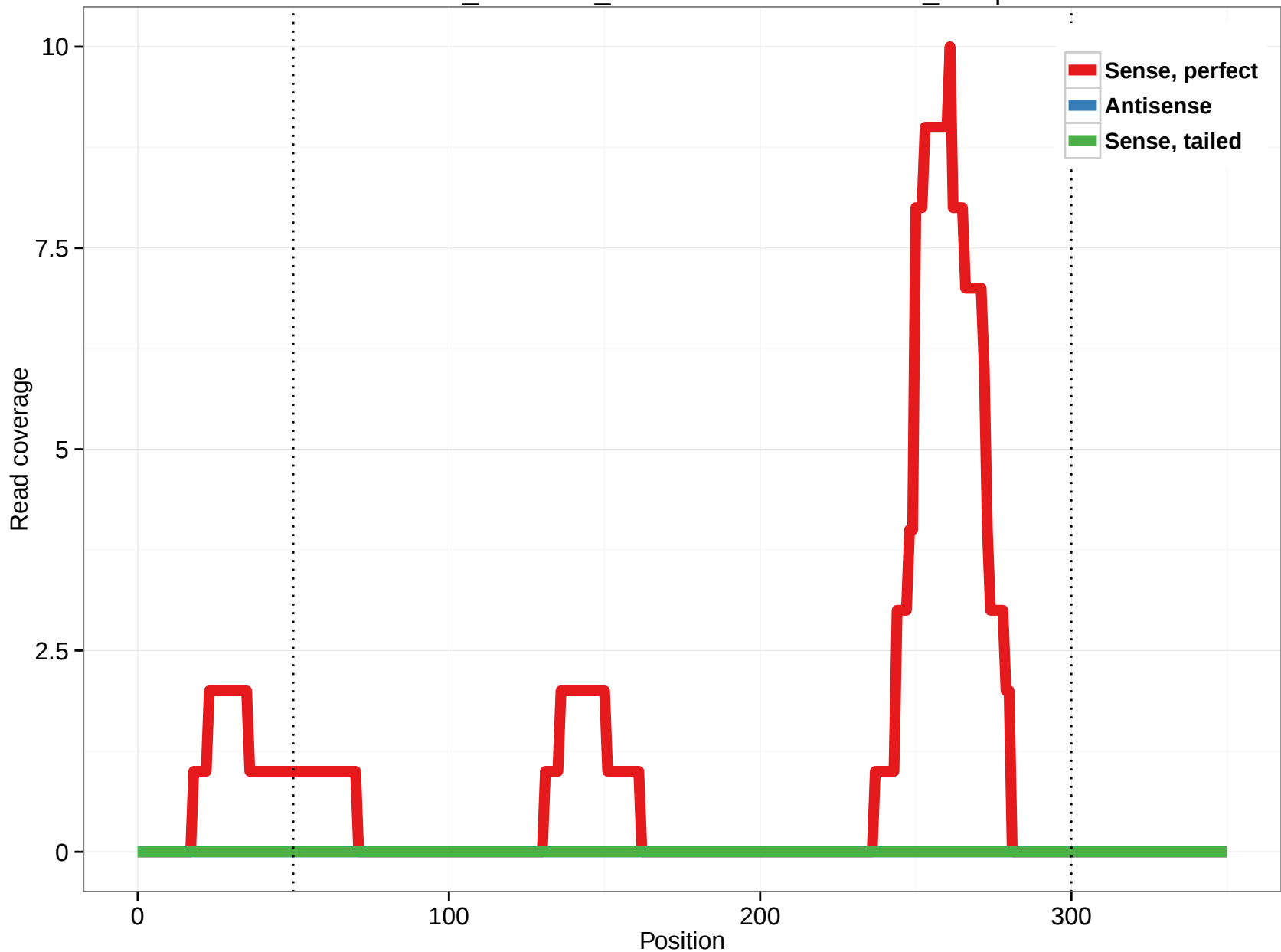
ornAna1_ensGene_ENSOANT00000009016_18.5p
