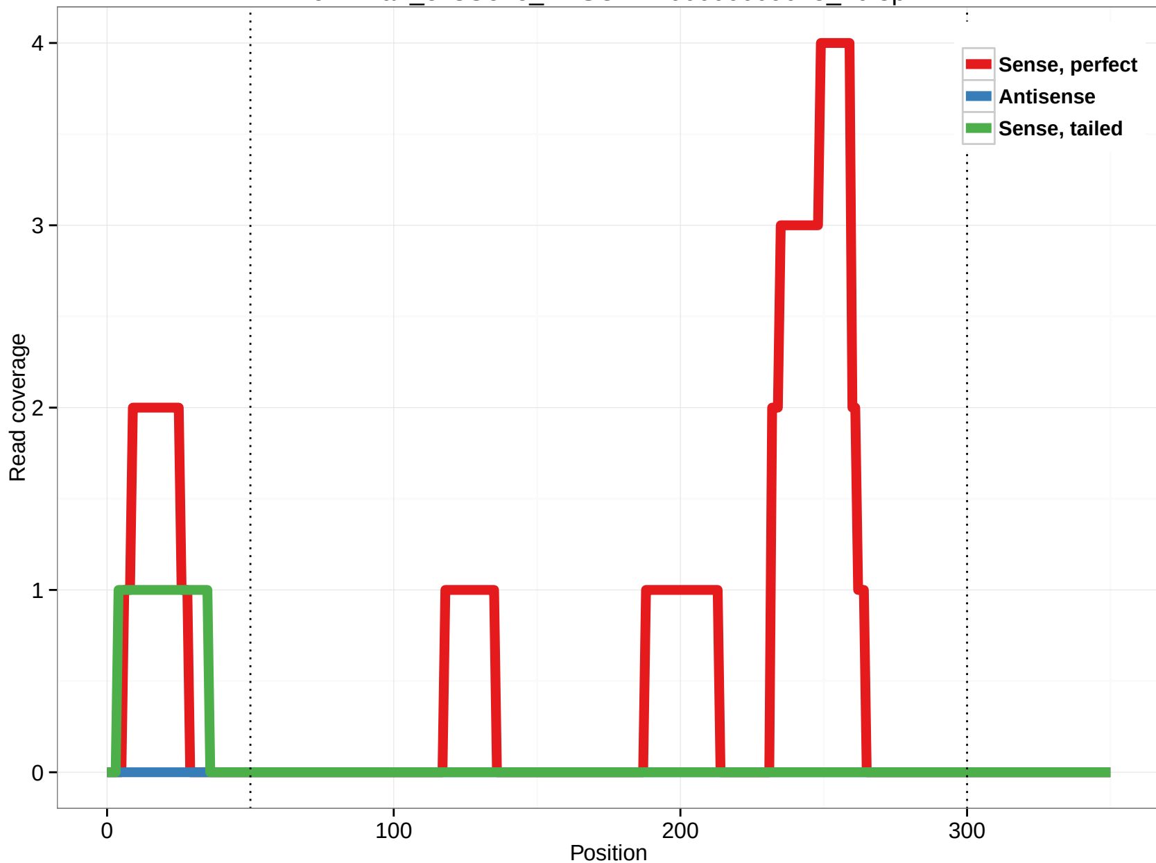
ornAna1_ensGene_ENSOANT00000009015_20.3p
