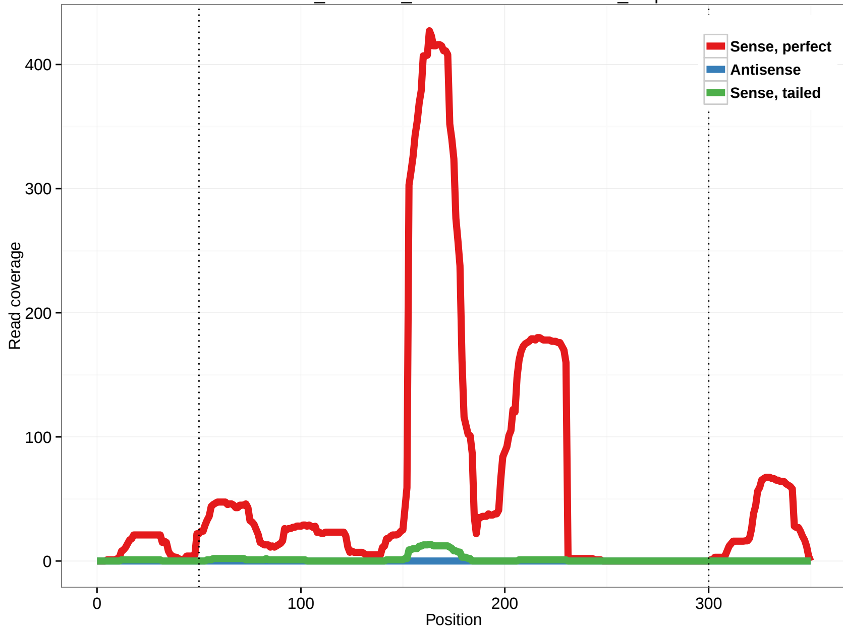
ornAna1_ensGene_ENSOANT00000008902_2.3p
