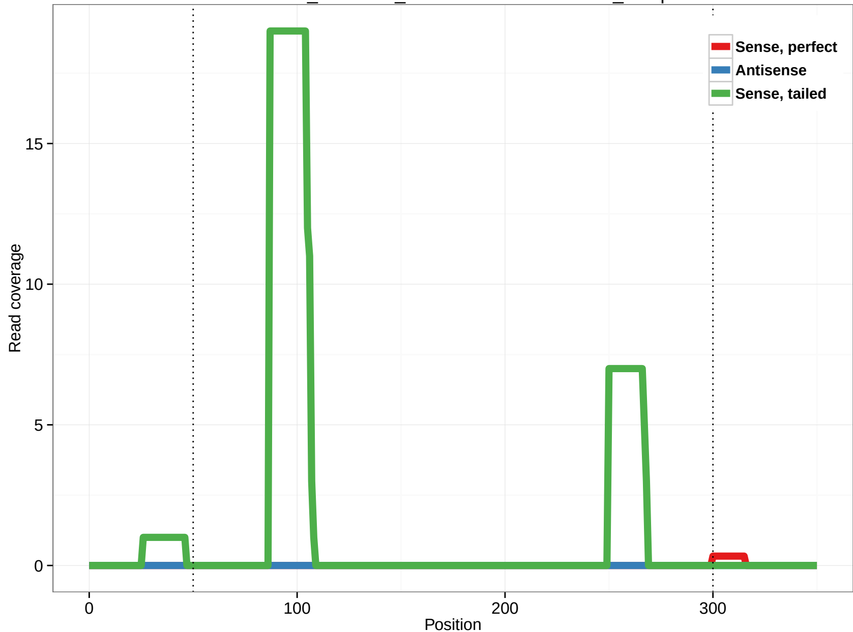
ornAna1_ensGene_ENSOANT00000008891_15.3p
