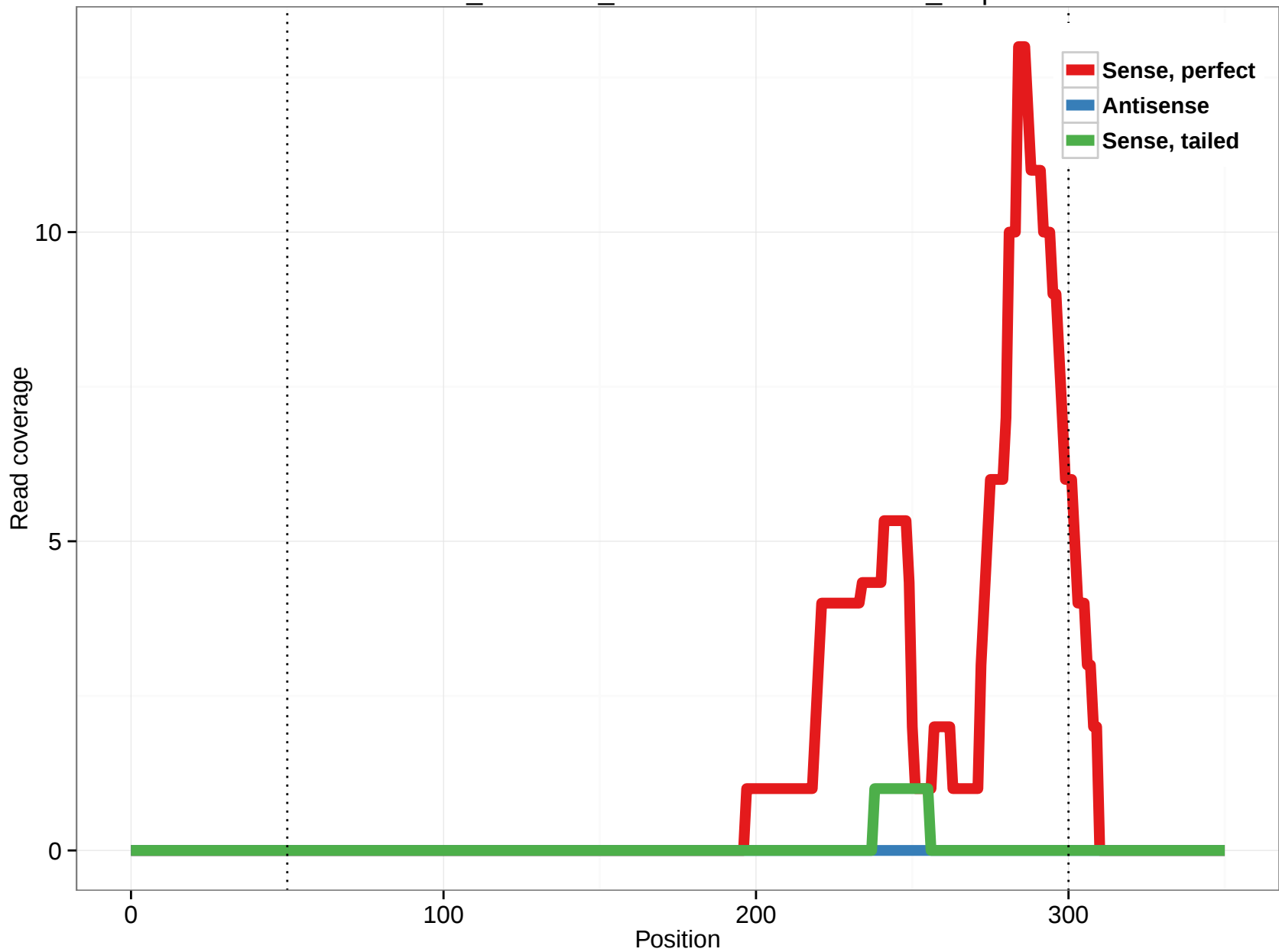
ornAna1_ensGene_ENSOANT00000008820_6.3p
