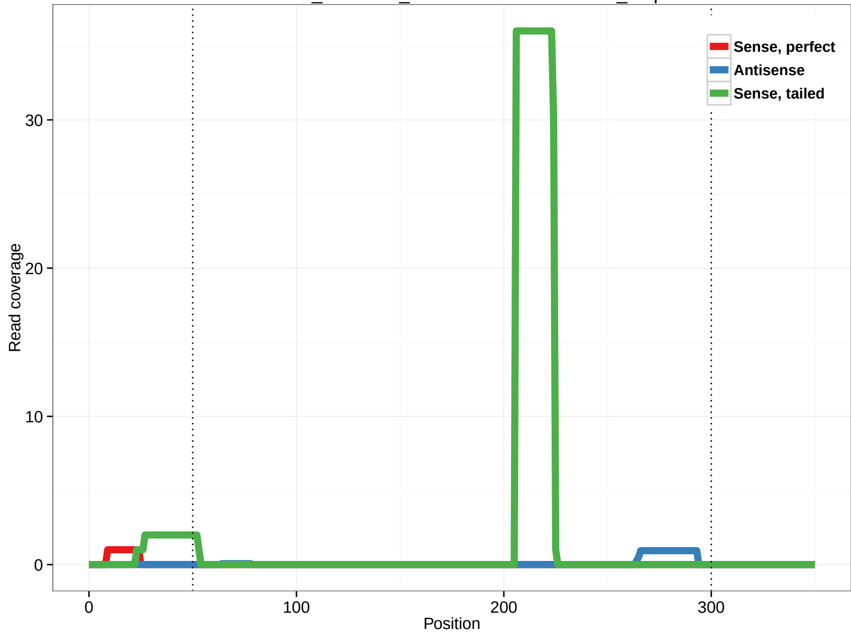
ornAna1_ensGene_ENSOANT00000008812_7.5p
