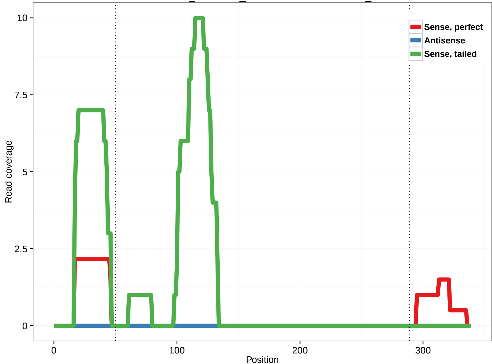
ornAna1_ensGene_ENSOANT00000008786_1
