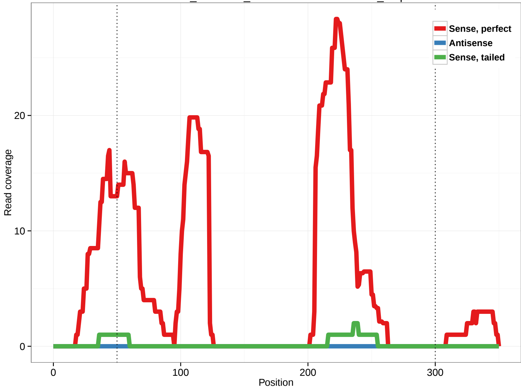
ornAna1_ensGene_ENSOANT00000008765_4.3p
