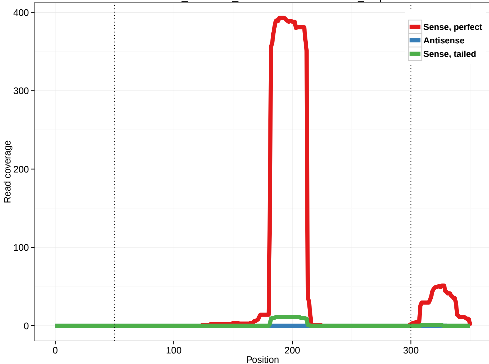
ornAna1_ensGene_ENSOANT00000008746_0.3p
