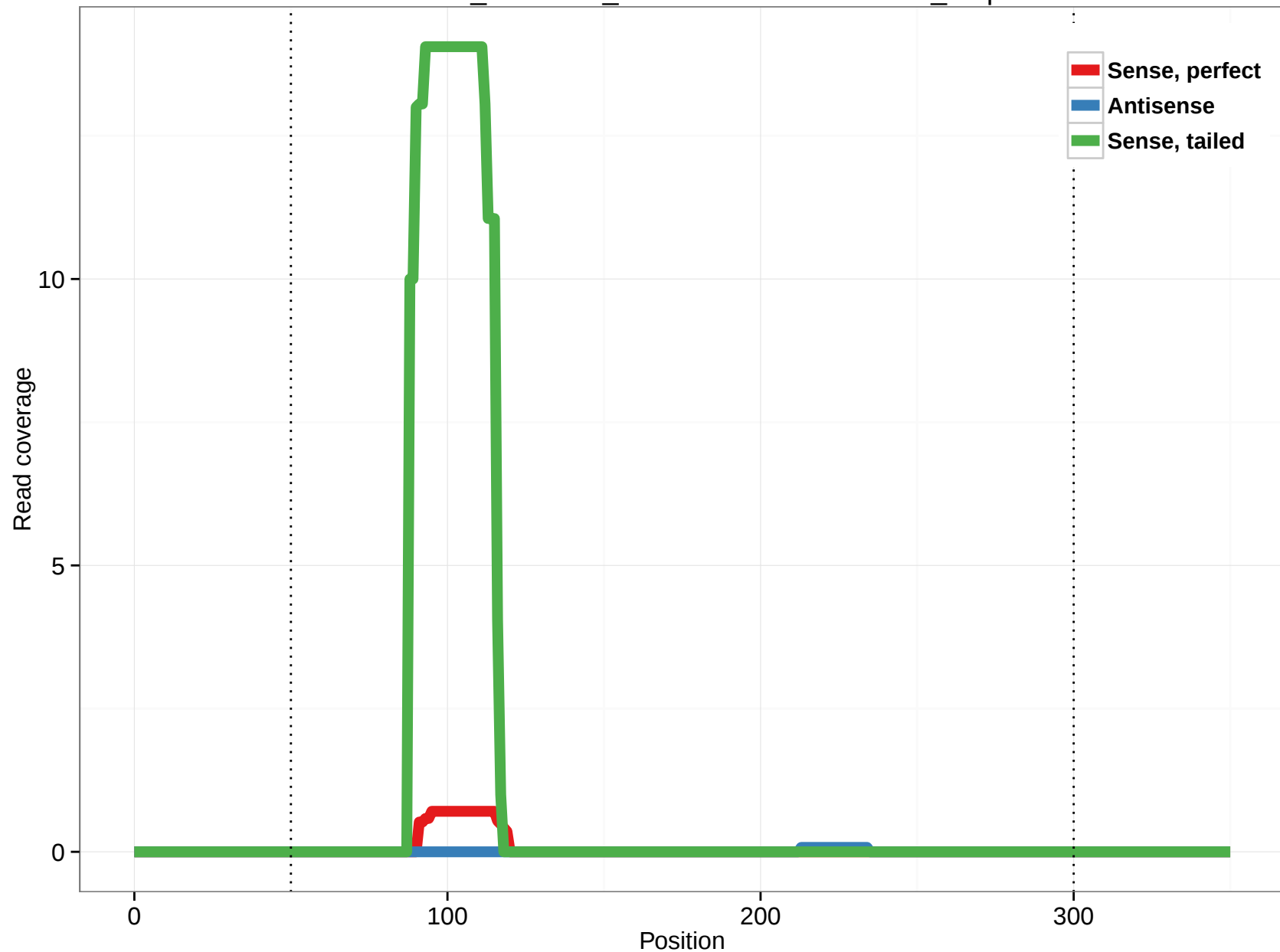
ornAna1_ensGene_ENSOANT00000008721_1.3p
