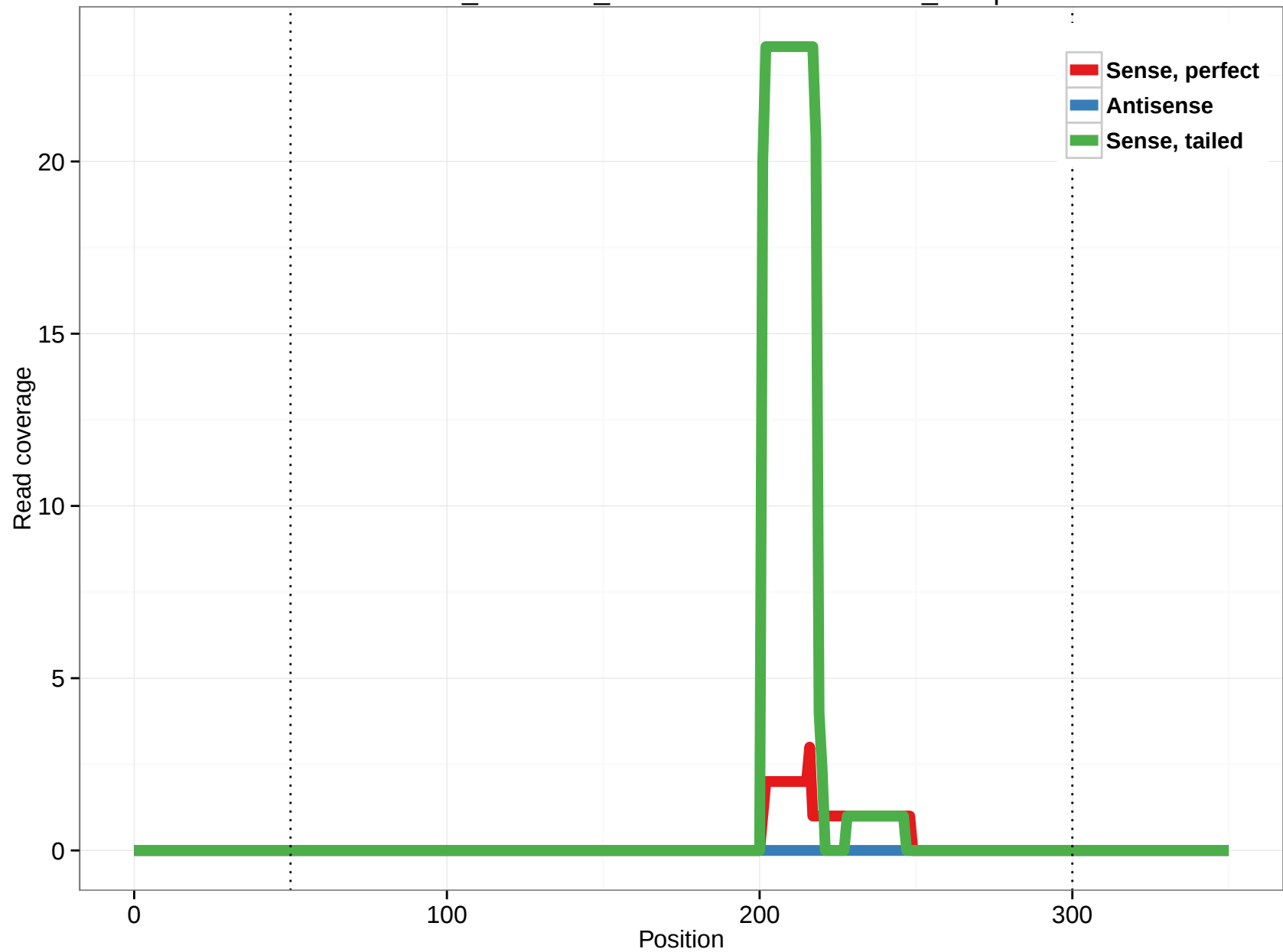
ornAna1_ensGene_ENSOANT00000008696_50.3p
