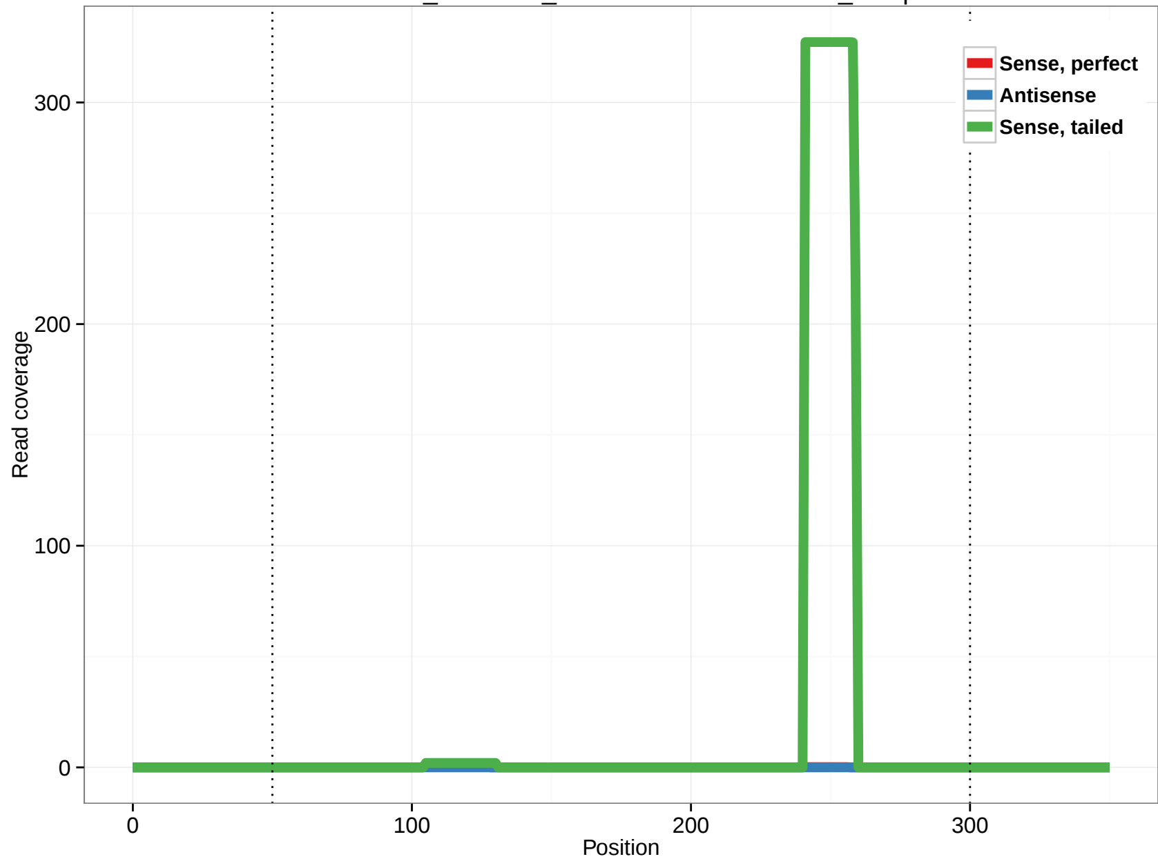
ornAna1_ensGene_ENSOANT00000008691_12.5p
