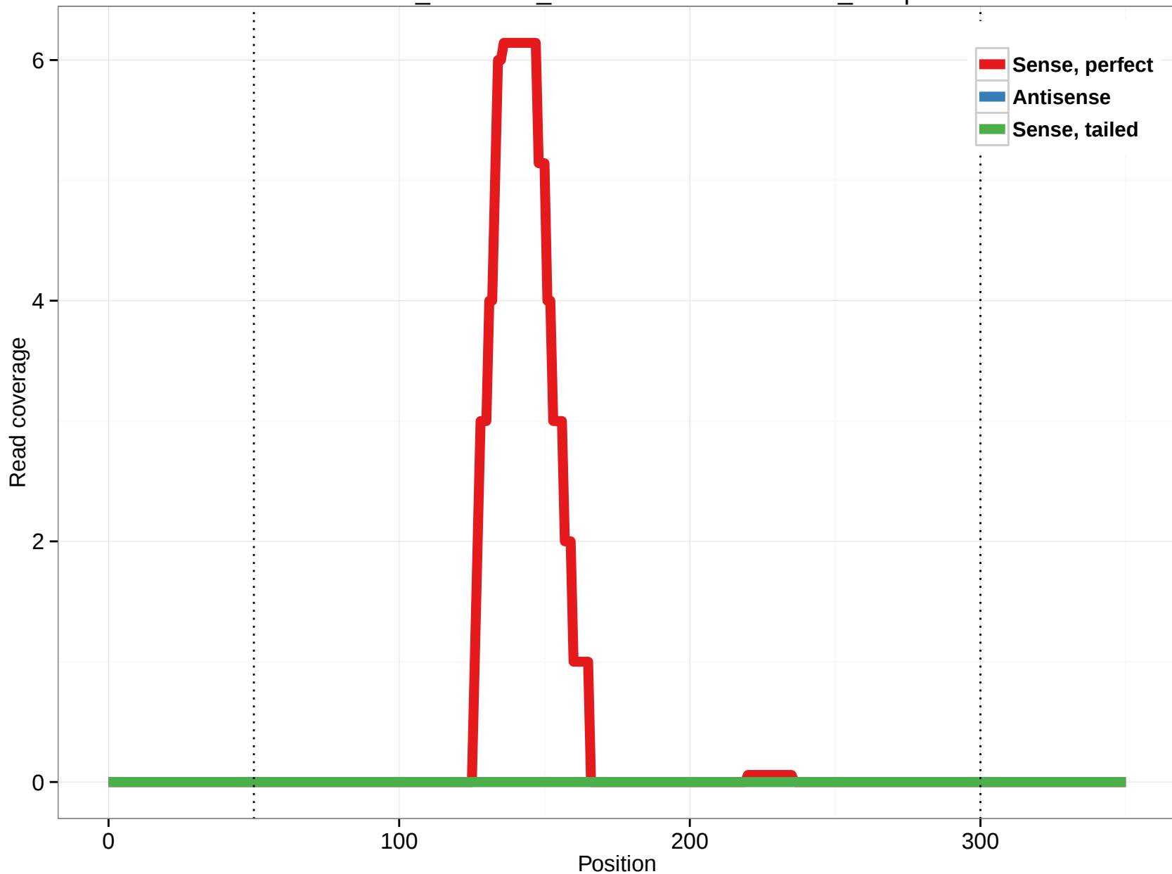
ornAna1_ensGene_ENSOANT00000008684_15.3p
