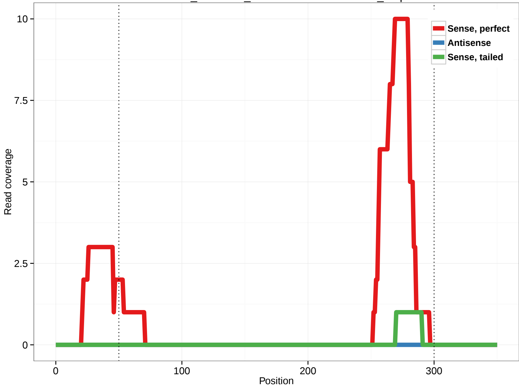
ornAna1_ensGene_ENSOANT00000008683_6.3p
