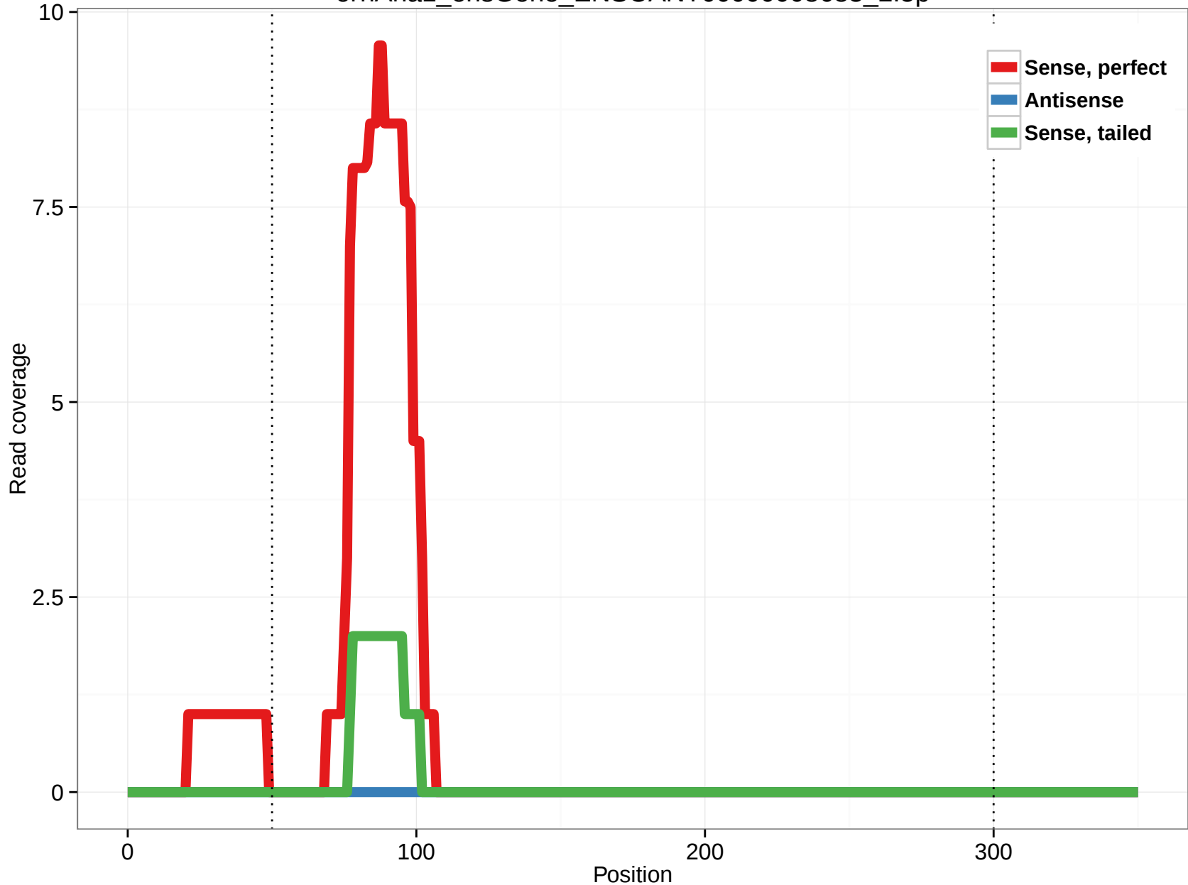
ornAna1_ensGene_ENSOANT00000008683_2.5p
