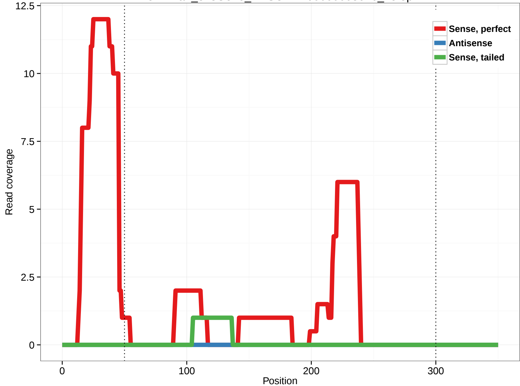
ornAna1_ensGene_ENSOANT00000008676_25.5p
