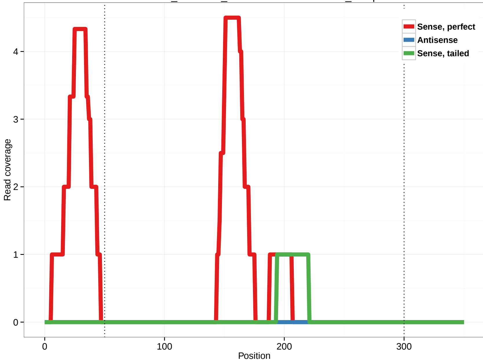
ornAna1_ensGene_ENSOANT00000008676_16.5p
