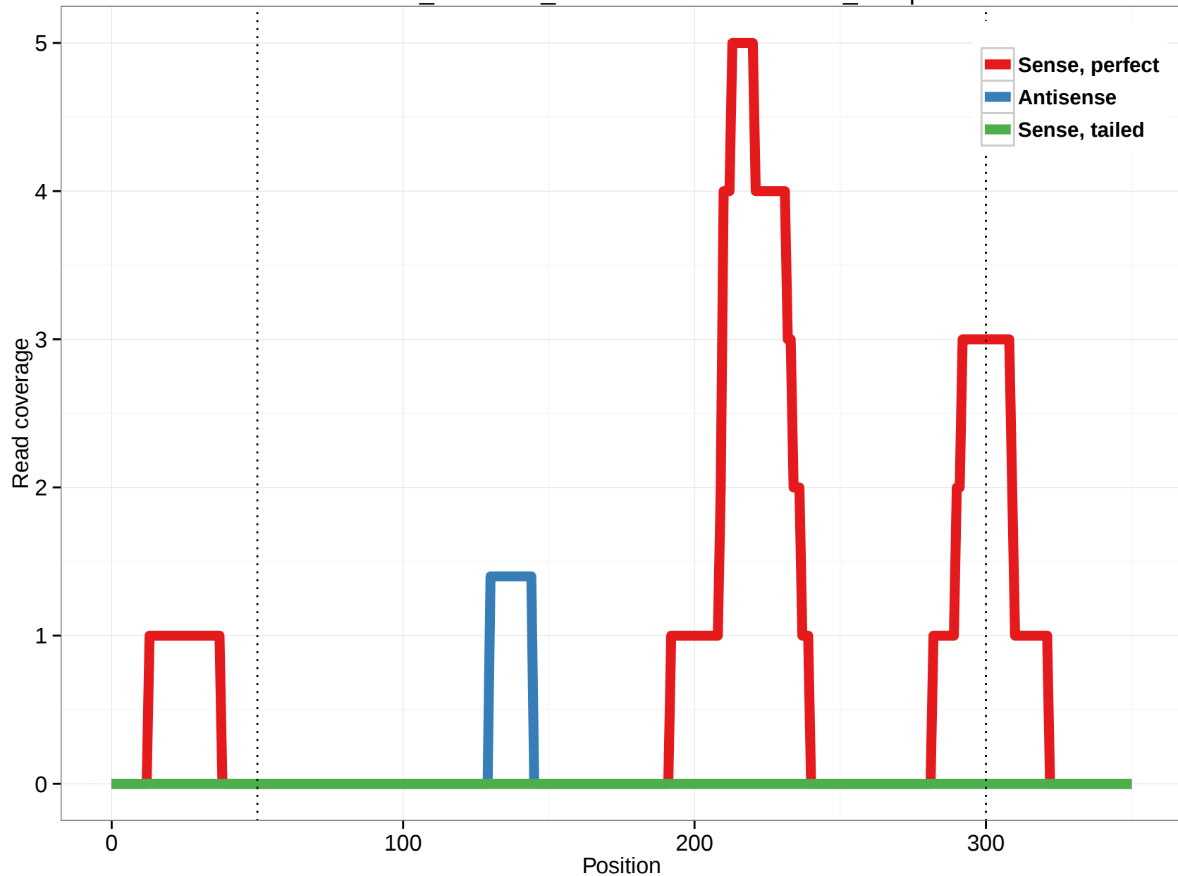
ornAna1_ensGene_ENSOANT00000008676_15.5p
