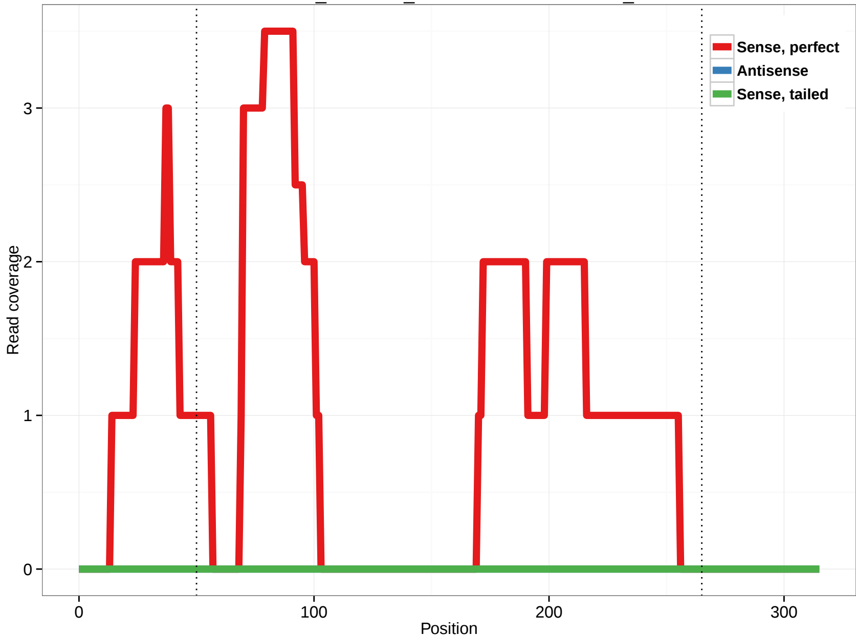
ornAna1_ensGene_ENSOANT00000008676_14
