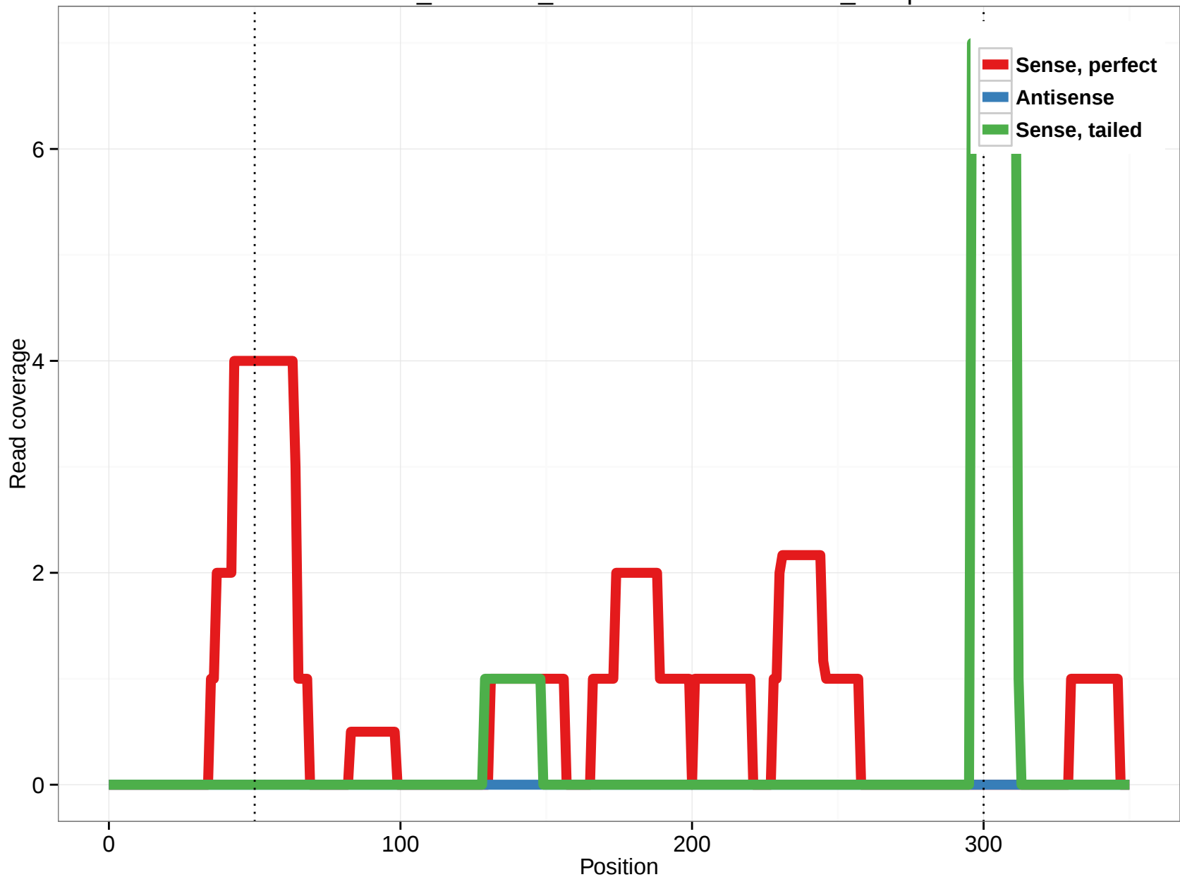
ornAna1_ensGene_ENSOANT00000008676_13.5p
