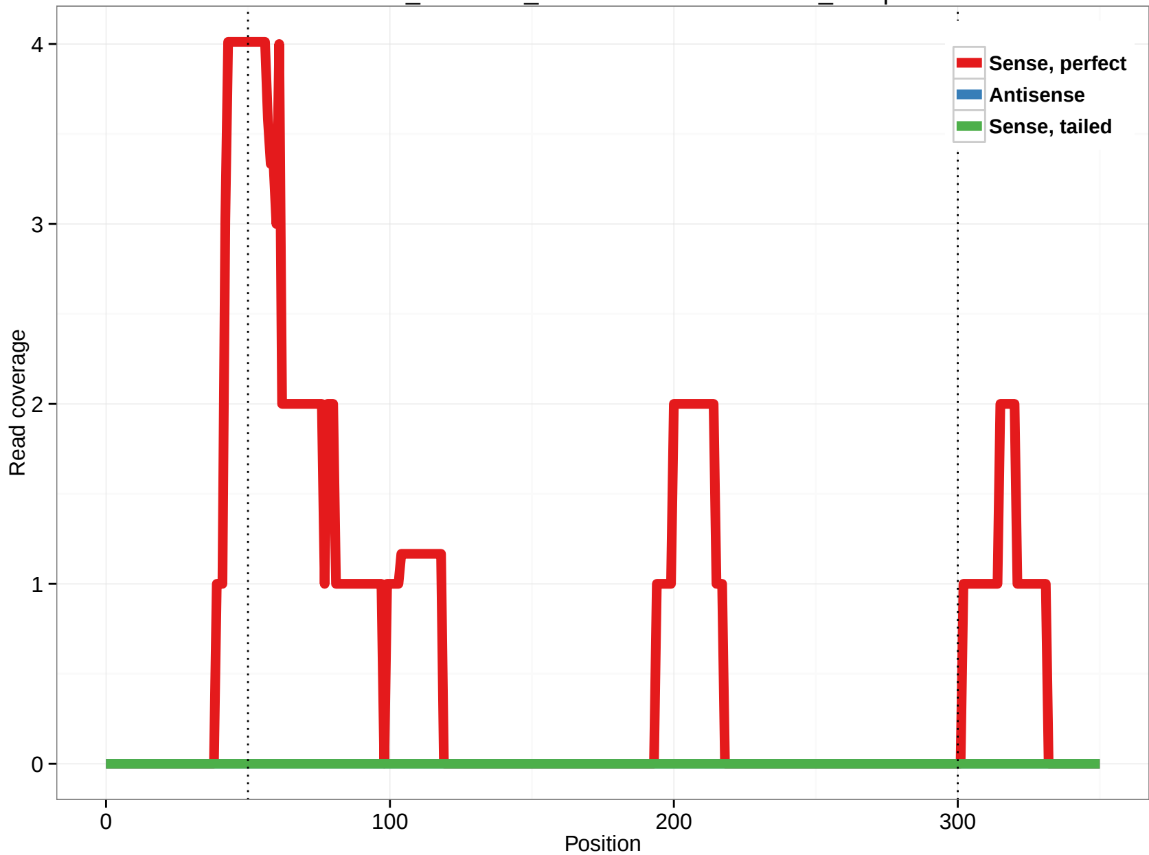
ornAna1_ensGene_ENSOANT00000008676_12.3p
