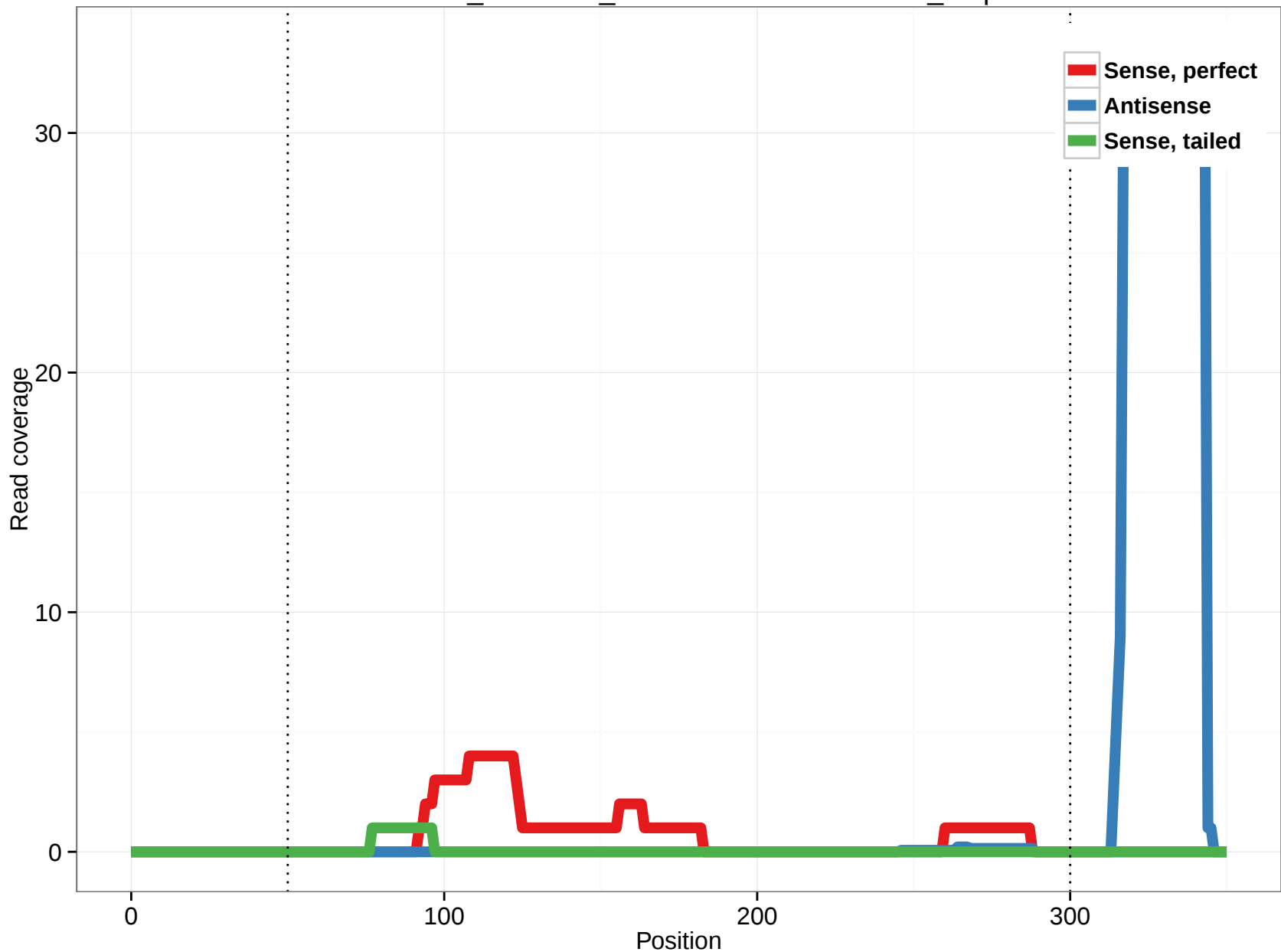
ornAna1_ensGene_ENSOANT00000008668_3.5p
