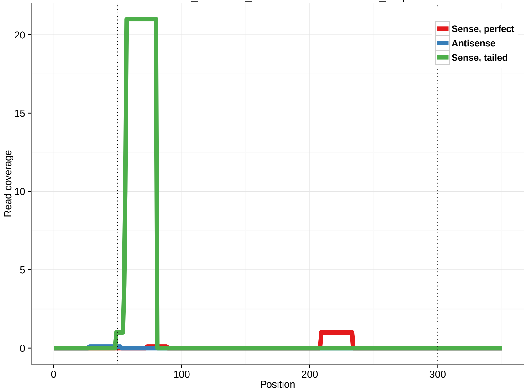
ornAna1_ensGene_ENSOANT00000008655_2.3p
