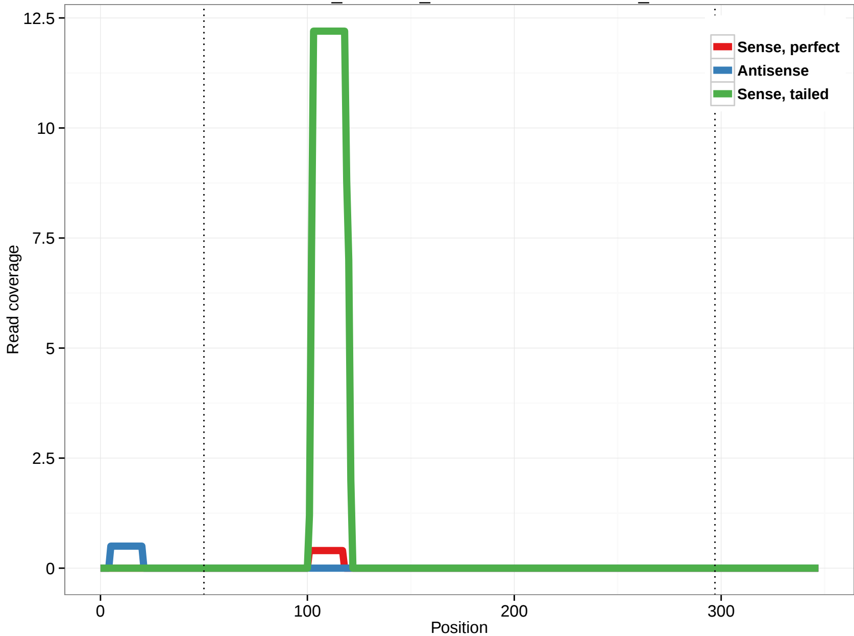
ornAna1_ensGene_ENSOANT00000008646_2
