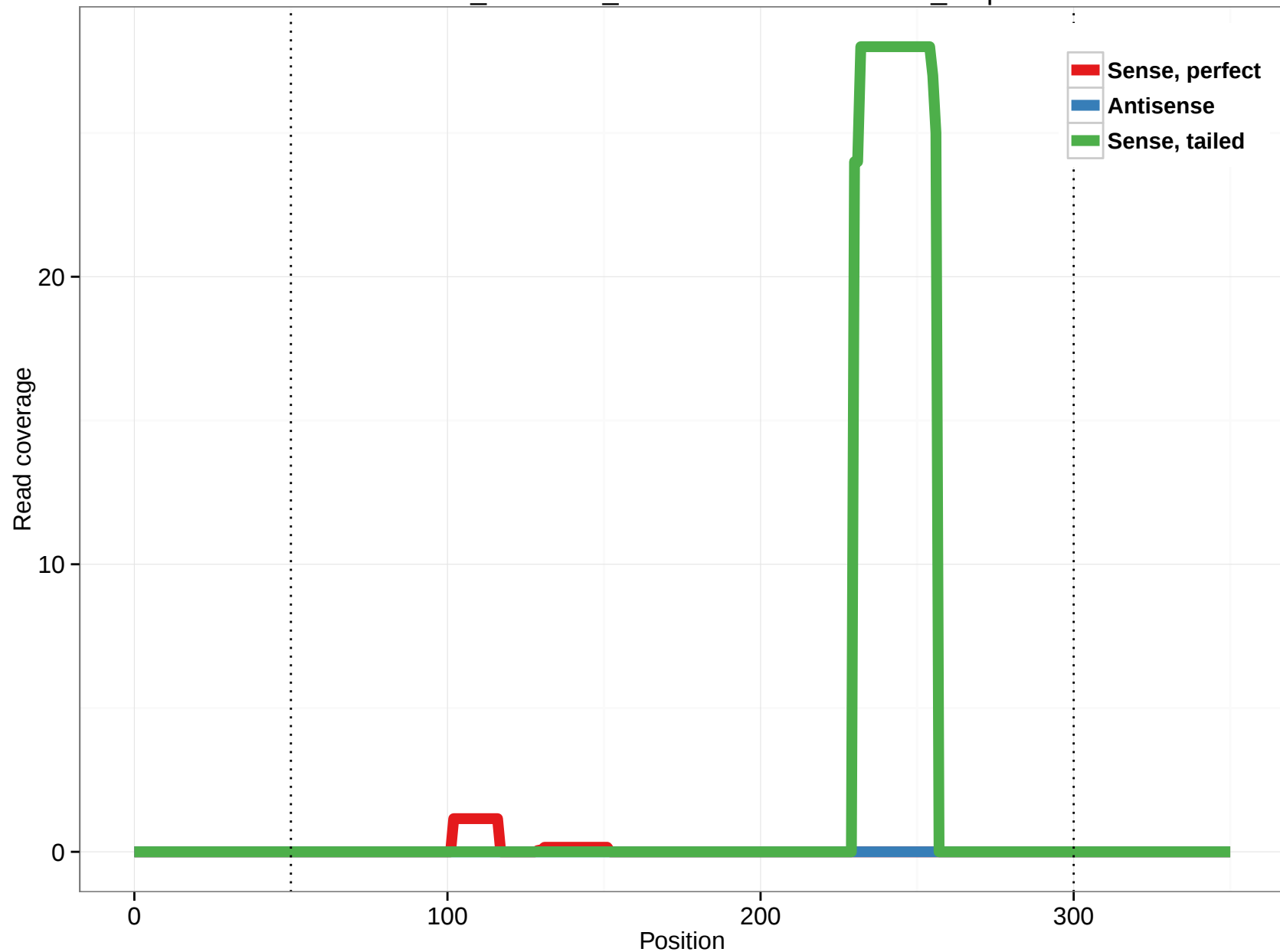
ornAna1_ensGene_ENSOANT00000008593_3.5p
