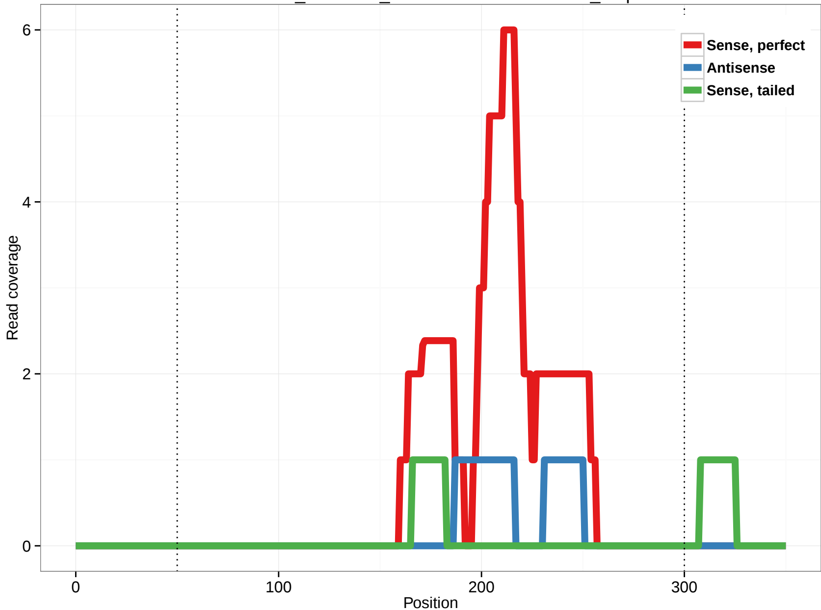
ornAna1_ensGene_ENSOANT00000008522_1.5p
