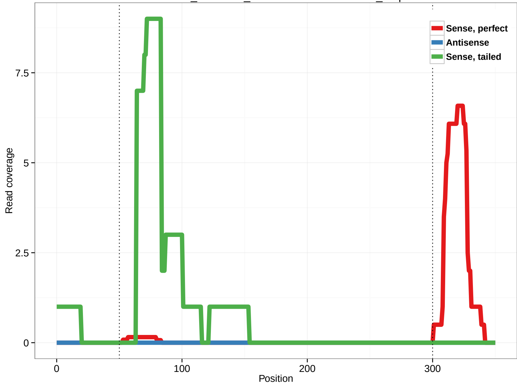
ornAna1_ensGene_ENSOANT00000008476_0.3p
