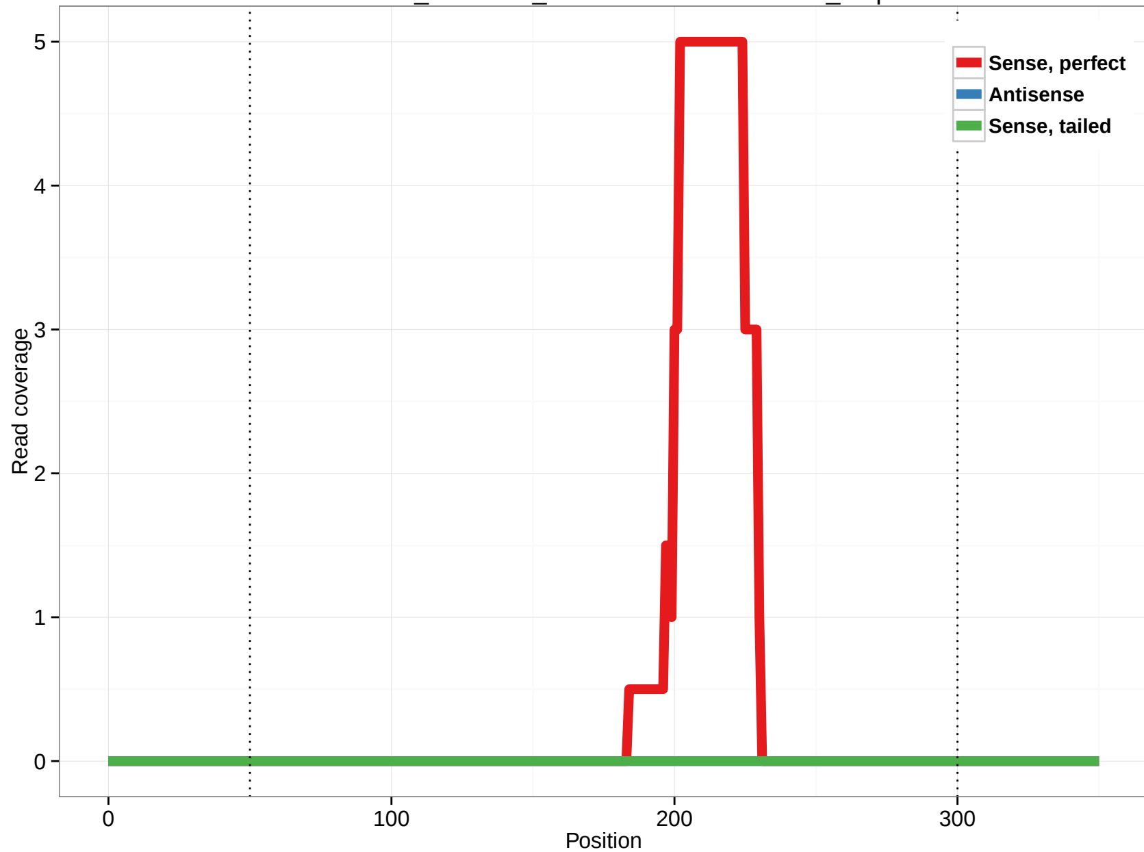
ornAna1_ensGene_ENSOANT00000008422_5.5p
