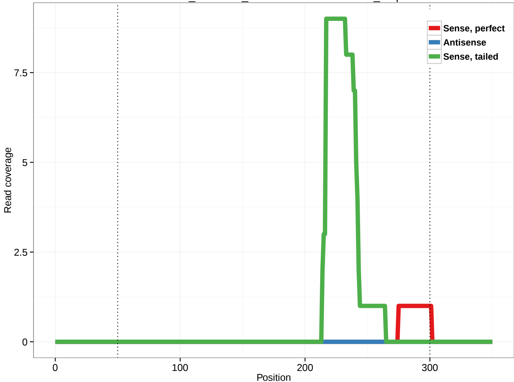
ornAna1_ensGene_ENSOANT00000008367_2.5p
