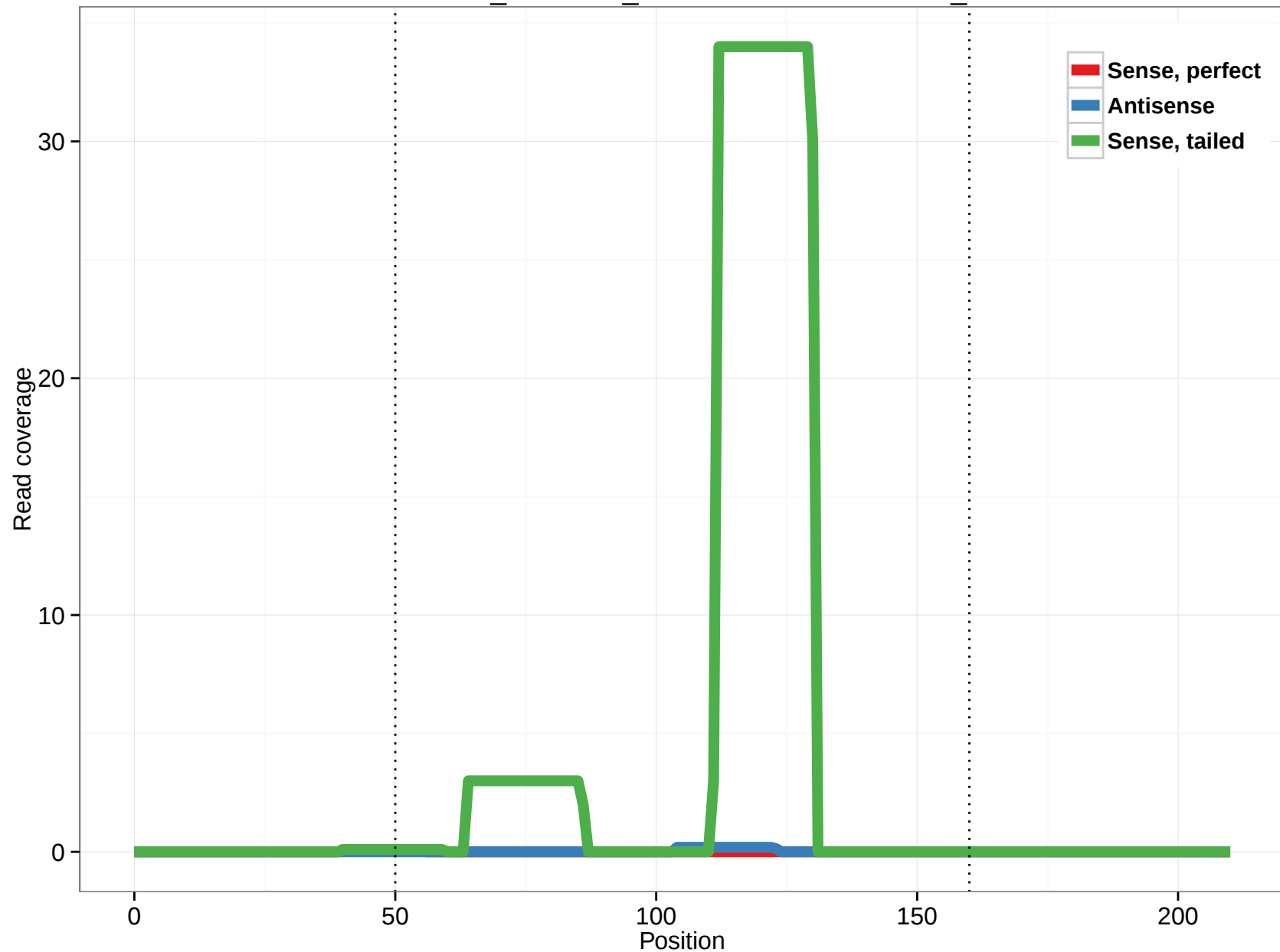
ornAna1_ensGene_ENSOANT00000008345_2
