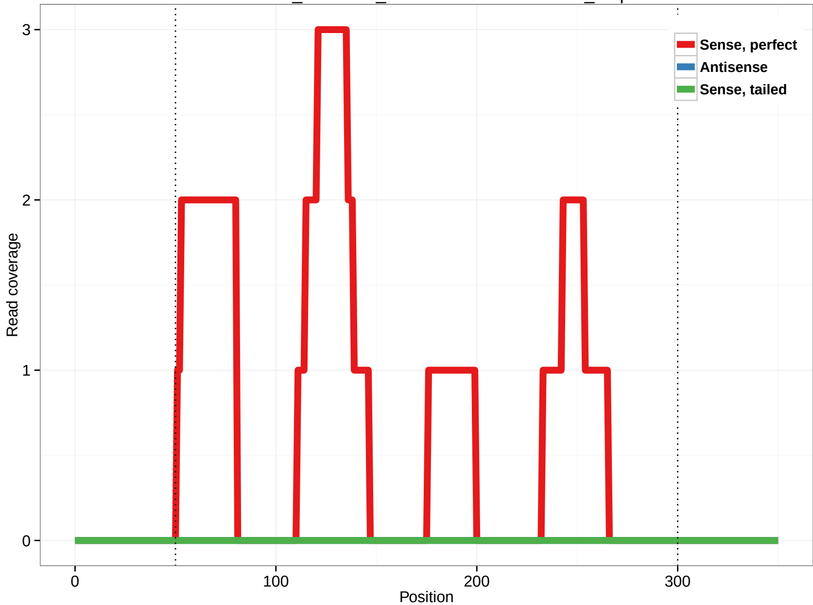
ornAna1_ensGene_ENSOANT00000008306_6.5p
