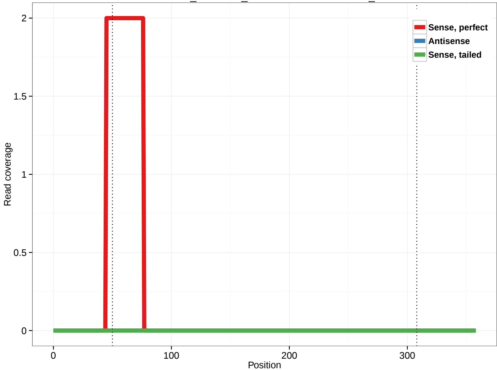
ornAna1_ensGene_ENSOANT00000008283_4
