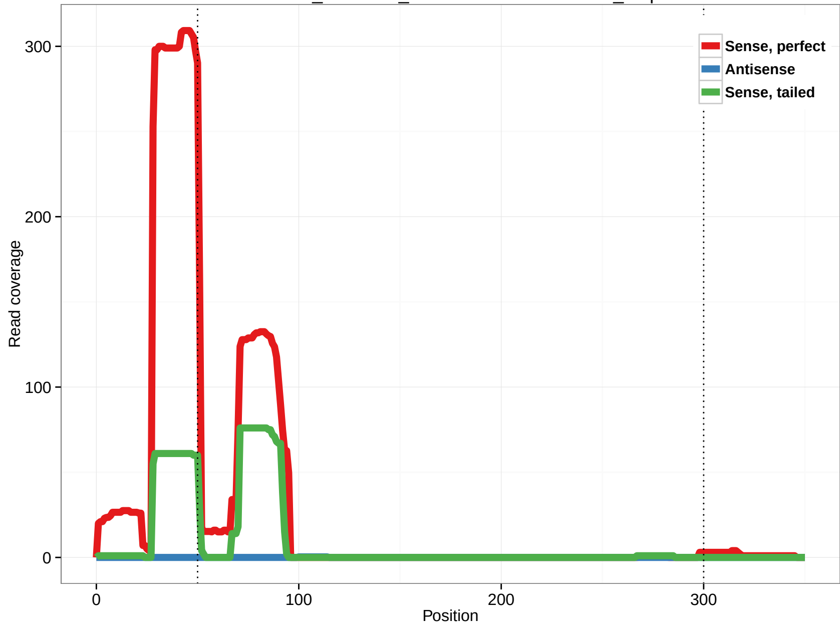
ornAna1_ensGene_ENSOANT00000008235_1.3p
