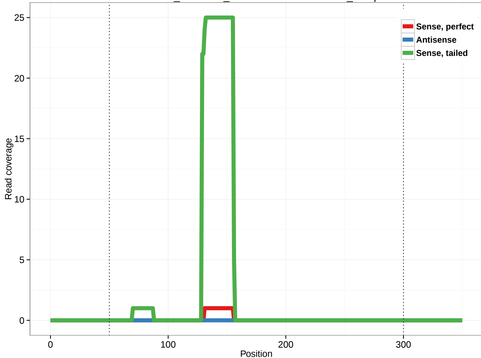
ornAna1_ensGene_ENSOANT00000008177_27.3p
