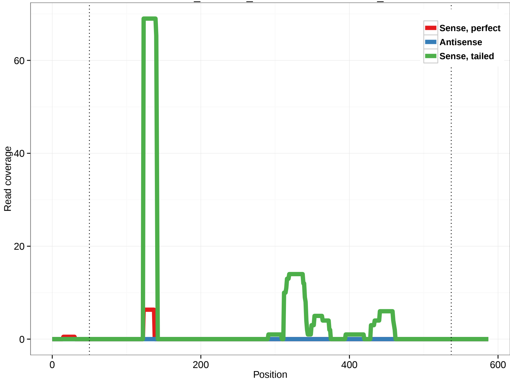
ornAna1_ensGene_ENSOANT00000008167_2
