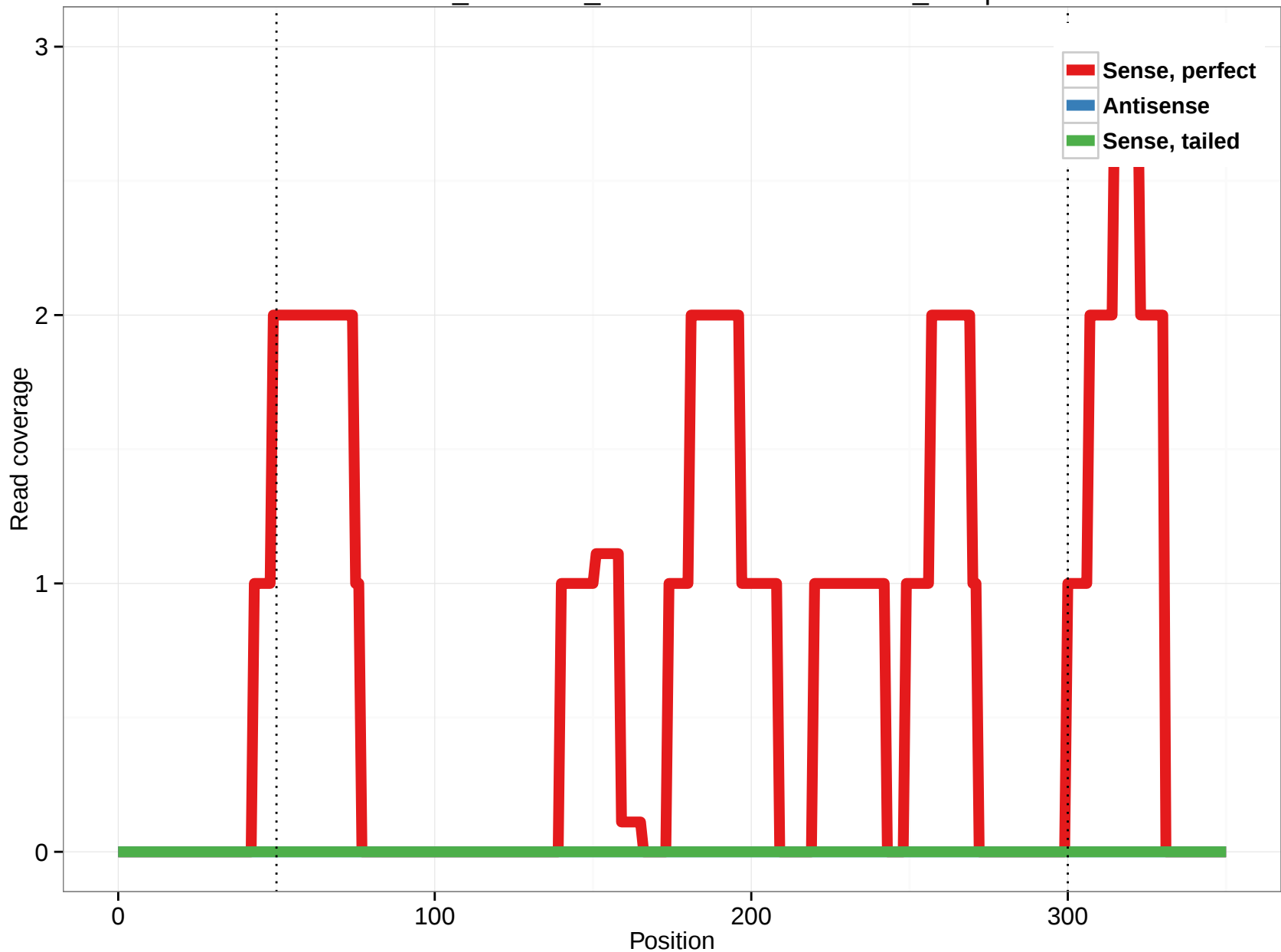
ornAna1_ensGene_ENSOANT00000008159_18.3p
